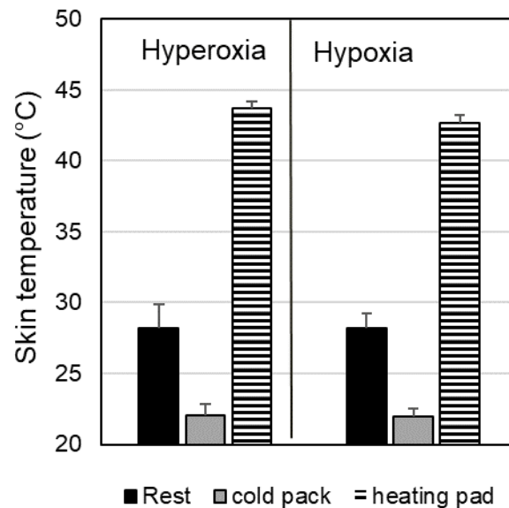
Figure 3. Skin temperature beside the TCM probe during temperature interventions, Data Set 1. Bars indicate one standard error.
