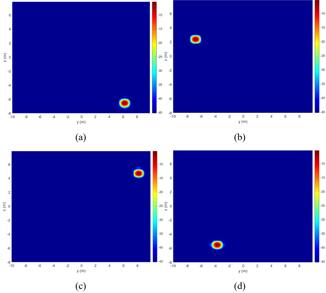
Fig. 13 Vertical y-z planar cuts through the 3-D PFA image obtained for the full FLSAR configuration after the WCEC procedure, at x coordinates corresponding to the four target image peaks: a) x = -8.125 m (Target 3), b) x = -5.937 m (Target 4), c) x = 5.937 m (Target 1), and d) x = 6.719 m (Target 2). The point target true coordinates are listed in Table 2.
