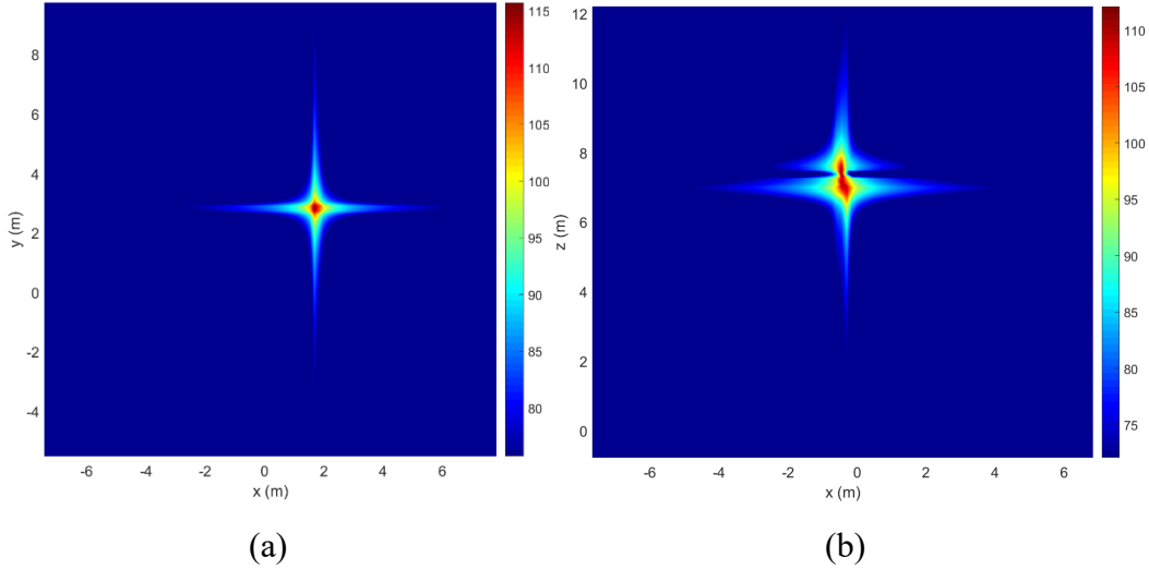
Fig. 9 Representation of the WCEC FIR filter impulse response magnitude for the 2-D imaging examples in Section 3.1: a) side-looking configuration (x-y plane), and b) forward-looking configuration (x-z plane). Both filters are designed for Target 1 in each of those numerical examples.
