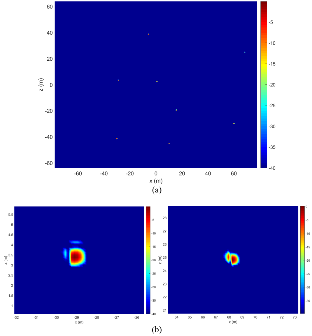
Fig. 12 2-D SAR image obtained by PFA and the WCEC procedure for the forward-looking geometry in the x-z plane for the same point target set as in Fig. 4, showing a) the full image and b) details around two targets exhibiting the split image issue. None of the other target images displays this issue.
