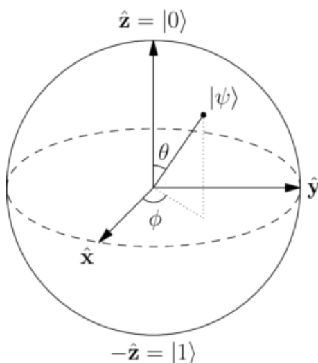
Bloch Sphere, a geometric representation of quantum superposition. Each qubit state is a point on the surface of the sphere. M
