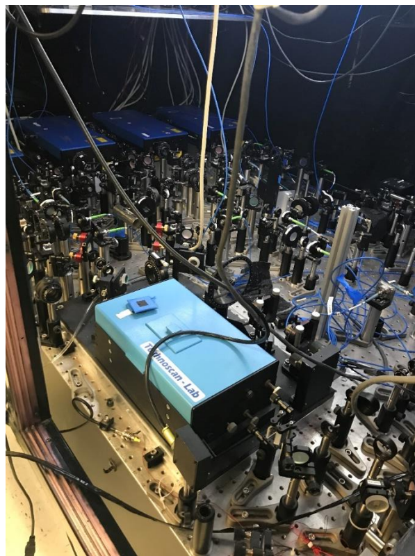
reaching early commercial market in 22. One of three light tables at SBU which is fully populated with equipment for testing and experiments. Note the new light tables at BNL are just now starting to be populated with lenses and devices so test and experiments can be setup. (Picture by Patrick Lancaster)
