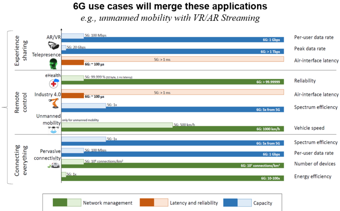
Representation of multiple KPIs of 6G use cases, together with the improvements with respect to 5G networks.
