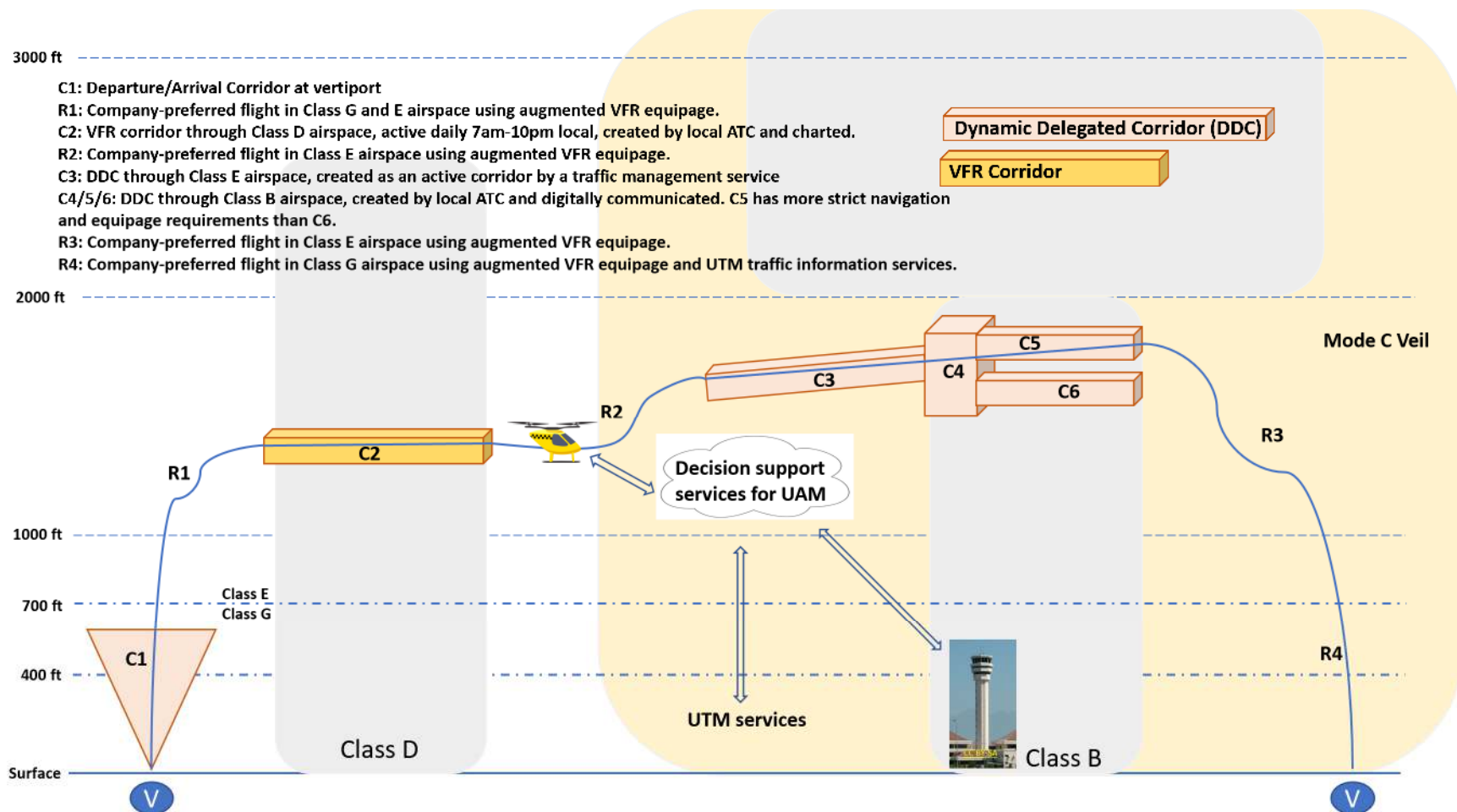
Figure 1: Notional Depiction of Airspace Integration Concepts
