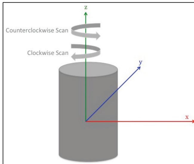
Figure 4-1. LiDAR coordinate system.
