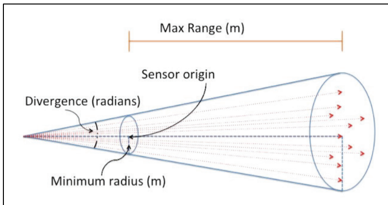
Figure 4-2. Ray sampling of LiDAR pulse.
