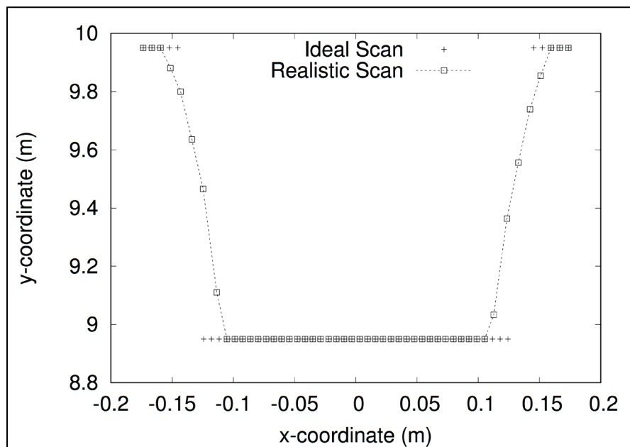
Figure 4-4. Example VANE LiDAR scans with and without beam divergence.
