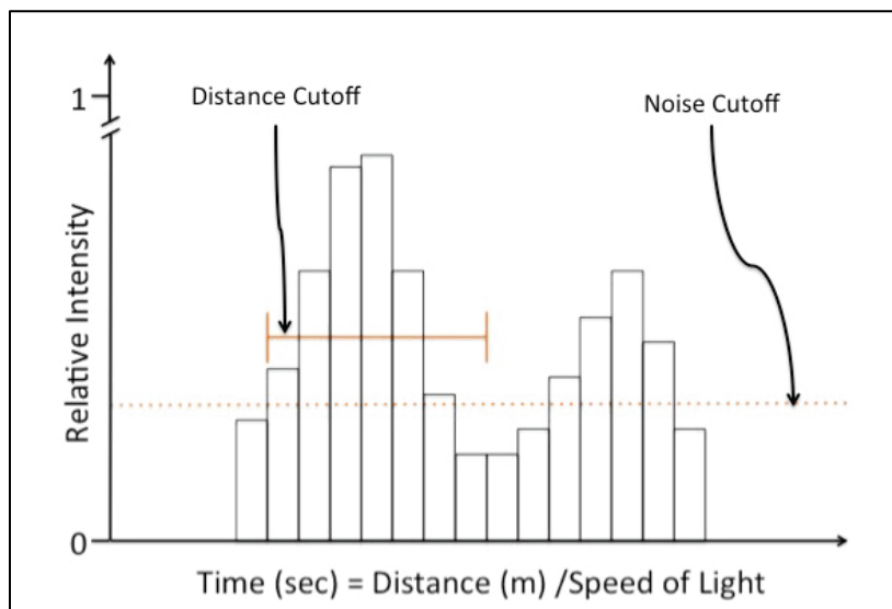
Figure 4-3. Example of LiDAR signal processing algorithm used in VANE.
