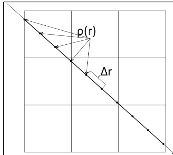
Figure 8-1. 2-D illustration of the volume rendering algorithm in VANE.
