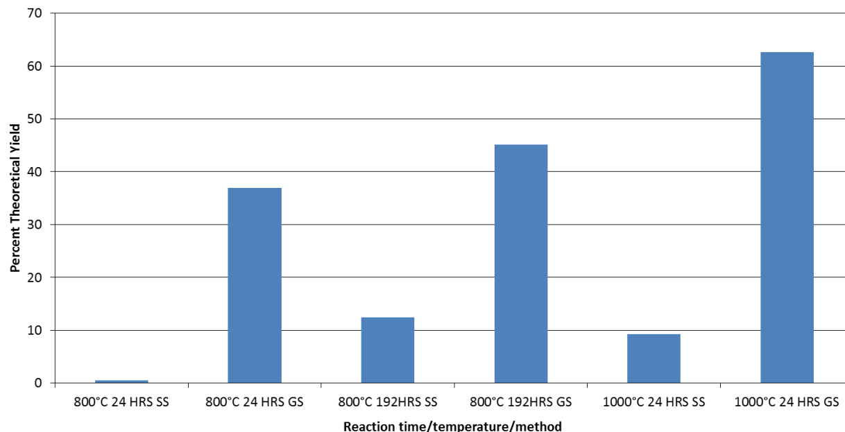
Figure 17: Extent of reactive conversion of (\text{Ti}_{0.77}\text{W}_{0.23})\text{C} into \text{TiC} and \text{W} for gas-solid and solid-state reactions at the specified process conditions.
