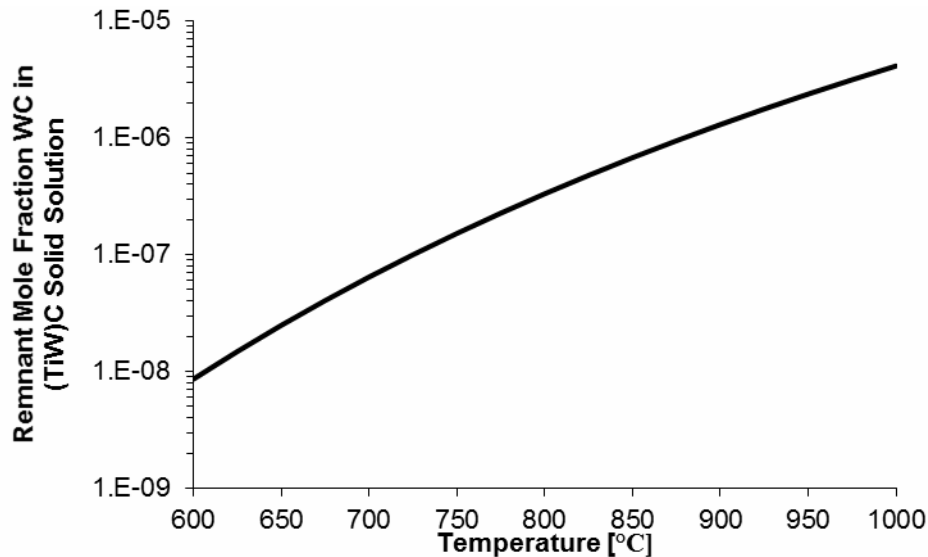
Figure 15: Equilibrium remnant mole fraction WC in (Ti,W)C upon gas-solid reaction of (\text{Ti}_{0.77}\text{W}_{0.23})\text{C} with excess titanium. Calculated using FactSAGE 6.4 assuming ideal solid solution behavior of the mixed carbide phase.
