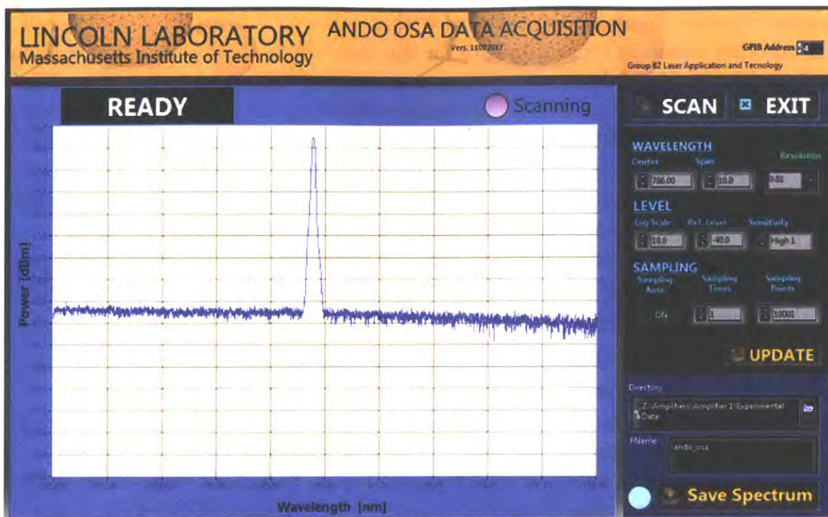
Figure 4-3: Pulsed laser diode (786nm Lumics LU0786M100-1G06E10A with PicoLAS BFS-VRM-03HP driver) spectrum analysis screenshot.
