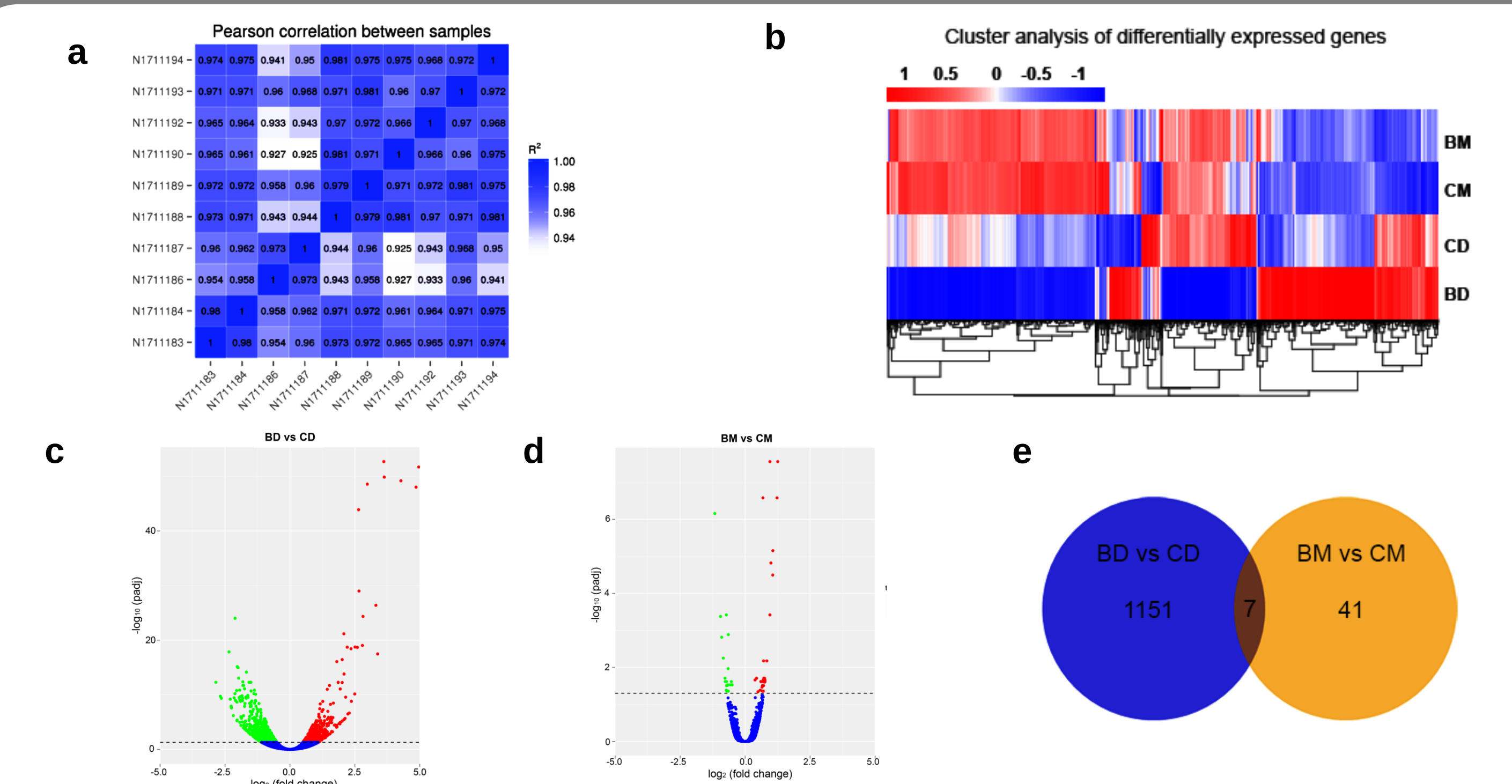
Figure 4. Heat maps and cluster analysis of gene expression differences. (a) The correlation coefficient between samples. (b) In hierarchical clustering, areas of different colors denote different groups (clusters) of genes. The color range from red to blue represents the log 10 (FPKM+1) value from large to small. Experimental groups were CD (control, 1d), CM (control, 28d), BD (blast exposure, 1d) and BM (blast exposure, 28d). (c, d) Volcano plots showed the overall DEGs significant up (red) and down (blue) regulated genes. The threshold was set |log 2 (Fold change)| > 1 and padj < 0.05. (e) Venn diagram of the number of GEGs.
