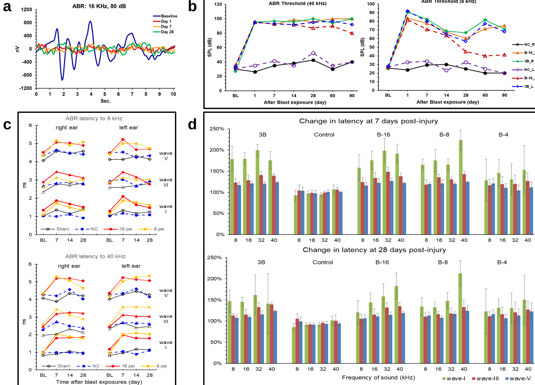
Fig. 2. ABR impairment following blast exposure. (a) Reduction in wave amplitudes after blast exposure, (b) elevation in thresholds to the sound of 8 and 40 KHz stimuli, (c) latency changes in the wave I, III and V, (d) changes in ratio of latency that compared to its baseline among experimental groups.
