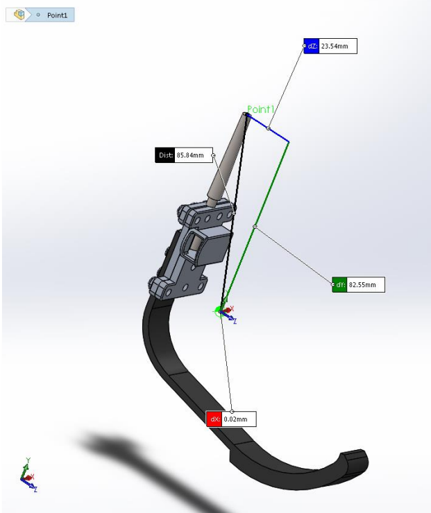
Figure 1. COM location and coordinate frames of passive transtibial prosthesis
