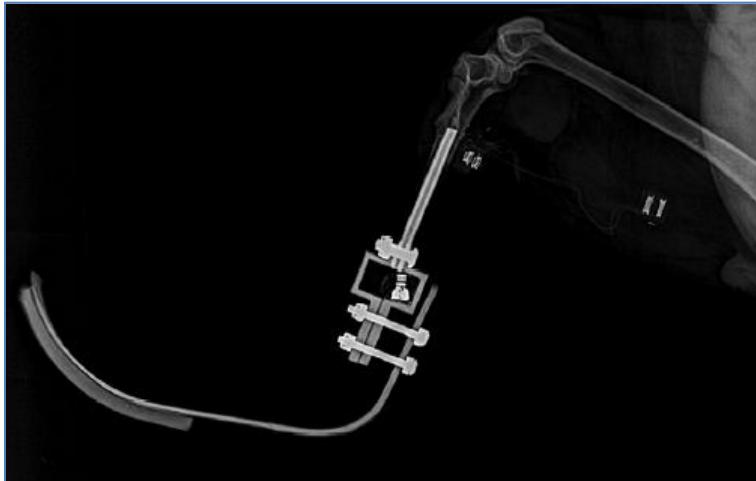
Figure 3. X-ray image of the SBIP-PN implant with attached passive transtibial prosthesis. Nerve cuff electrodes on the distal tibial and sciatic nerves with their leads and leads from muscle electrodes in the residual soleus and tibialis anterior muscles can be seen. The electrode leads were passed through the tibia and implant and secured with a connector in the aluminum chamber. The passive prosthesis can be substituted with a powered one. The connector will be used to transmit myoelectric signals and electrical stimulation trains between the prosthesis and muscles and sensory nerves.
