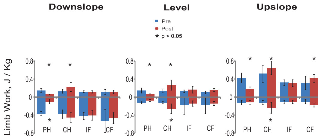
Fig. 5. Normalized negative and positive work done by four limbs during the cycle of pre (Pre) and post implantation (Post) walking in downslope (−50%), level (0%), and upslope (+50%) conditions. Mean (±SD) data of 4 animals. PH, right hindlimb (prosthetic hindlimb in Post condition); CH, contralateral hindlimb; IF, ipsilateral forelimb; CF, contralateral forelimb. Asterisks indicate significant differences ( p < 0.05 ) between pre and post implantation conditions.
