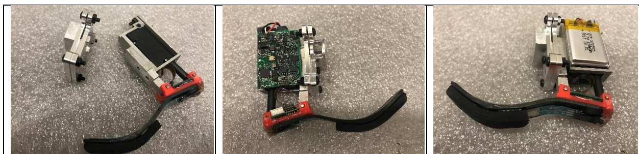
Figure 5. The powered prosthesis inside the holding frame. Left panel demonstrates the pylon holding plates (see Fig. 1) and the frame with a linear actuator and foot attached to the holding plates at the prosthetic joint. Middle panel shows a circuit board fixed to the right side of the linear actuator. The board includes a microprocessor unit, EMG amplifier, current stimulator and power management. Right panel shows the battery attached to the left side of
