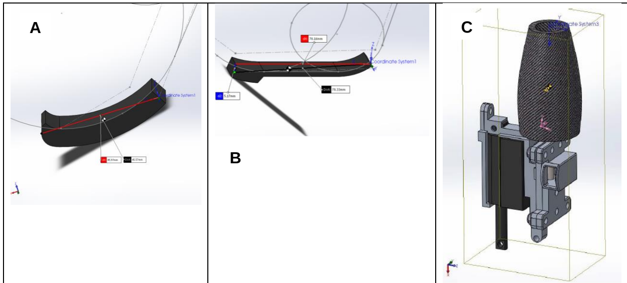
Figure 2. COM location and coordinate frames of the digits (A), tarsals (B) and shank (C) of the powered transtibial prosthesis
