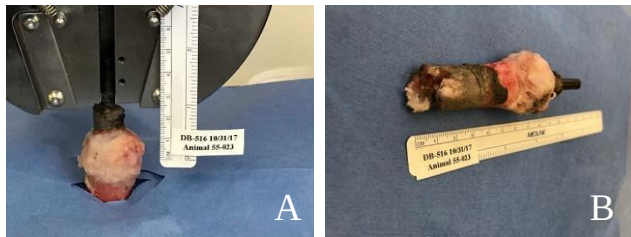
Figure 3. Mechanical Test. A - Pull-out test set up. B - Failure Mode: Bone fractured at holding pins. Implant to bone interface remained intact.
