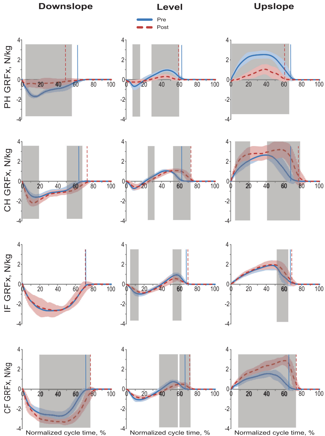
Fig. 3. Normalized tangential ground reaction forces (GRFx) during the cycle of pre implantation (Pre) and post implantation (Post) walking in downslope ( -50\% ), level ( 0\% ), and upslope ( +50\% ) conditions. Mean ( \pm SD) data of 4 animals. The vertical dashed and solid lines separate stance and swing phases for post and pre implantation, respectively. The shaded areas in each panel indicate significant difference ( p < 0.05 ) between the pre and post implantation walking determined using wANOVA analysis. PH, right hindlimb (prosthetic hindlimb in Post condition); CH, contralateral hindlimb; IF, ipsilateral forelimb; CF, contralateral forelimb.
