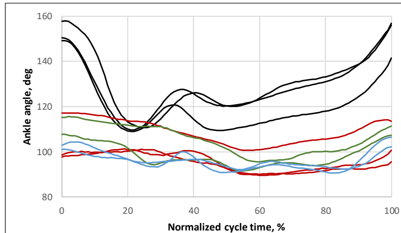
Figure 3. Ankle angles of representative cycles of one cat during level walking before amputation (black lines) and with powered transtibial prostheses with gear ratio 30 (blue lines), 63 (green lines) and 100 (brown lines). Cycle starts with swing onset, stance starts at ~35-40% in intact walking and at ~50-55% in prosthetic walking.
