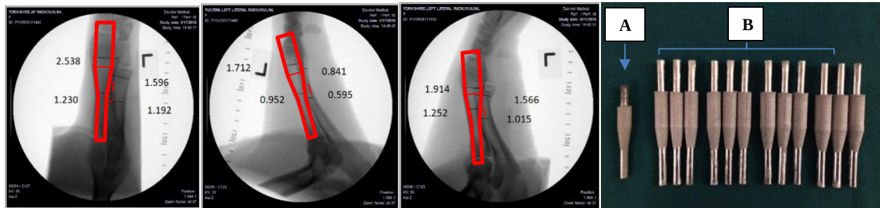
Figure 3. A fore limb implant dimensions and sizing. A - initial design SBIP-PNI; B - new SBIP-PNI pylons with elongated porous cladding.
