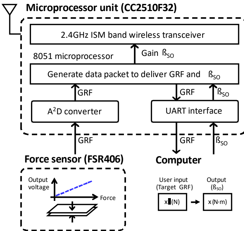
Figure 1. Detailed system block diagram of communications between the prosthesis and external devices (computer, force sensor and microprocessor unit). For details, see text.
