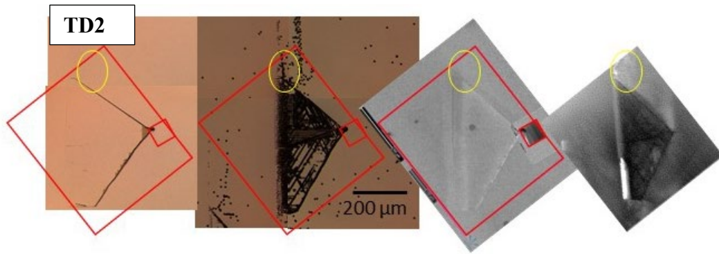
Fig. 5 Comparison of the optical microscopy, post-etch optical microscopy, SEM imaging, and CL imaging for the sample area denoted as TD2. The circled area shows contrast in the CL intensity within the SF where TEDs are located.
