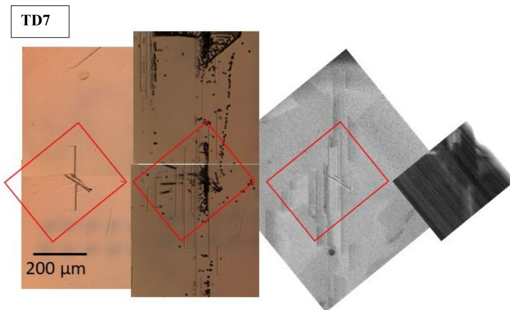
Fig. 9 Comparison of the optical microscopy, post-etch optical microscopy, SEM imaging, and CL imaging for the area on the sample denoted as TD7
