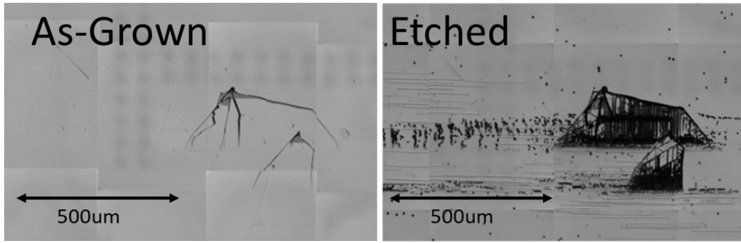
Fig. 1 Comparison of the as-grown and etched sample of SiC demonstrating how the TDs were used for image alignment
