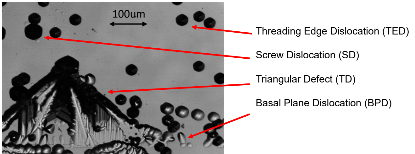
Fig. 3 The 4° off-axis 4H-SiC epitaxial layer etched for 10 min at 500 °C. Examples of a TED, SD BPD, and TD are all seen in this micrograph.
