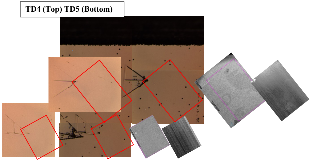
Fig. 7 Comparisons of the optical microscopy, post-etch optical microscopy, SEM imaging, and CL imaging for the sample areas denoted as TD4 and TD5
