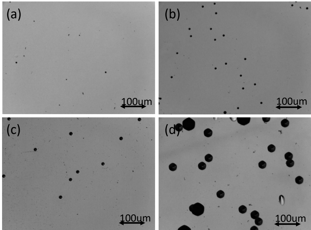
Fig. 2 Microscope images after KOH etching for a) 5 min 450 °C, b) 10 min 450 °C, c) 5 min 500 °C, and d) 10 min 500 °C
