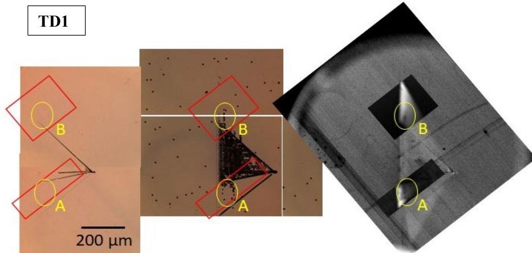
Fig. 4 Comparison of the optical microscopy, post-etch optical microscopy, SEM imaging, and CL imaging, for the sample area denoted as TD1. The circled areas show contrast in the CL intensity within the SF where TEDs are located.
