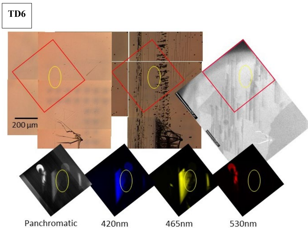
Fig. 8 Comparison of the optical microscopy, post-etch optical microscopy, SEM imaging, and CL imaging for the area on the sample denoted as TD6
