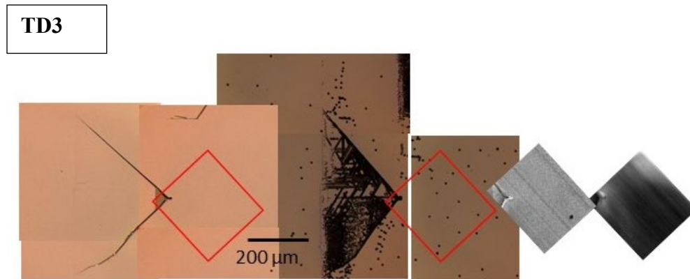
Fig. 6 Comparison of the optical microscopy, post-etch optical microscopy, SEM imaging, and CL imaging for the sample denoted as TD3
