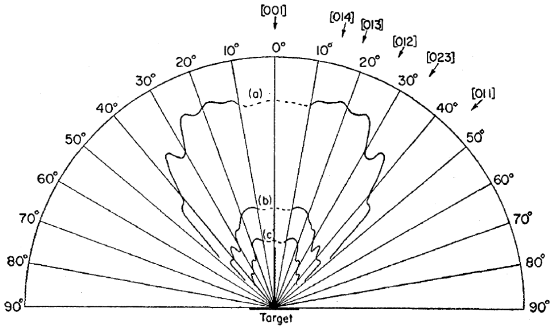
Figure 48: Angular distribution of secondary electrons from [001] face of copper crystal with 250 eV primary beam at normal incidence [111]. (a) 0 to 10 eV secondaries; (b) 10 to 20 eV secondaries; (c) 20 to 40 eV secondaries.
