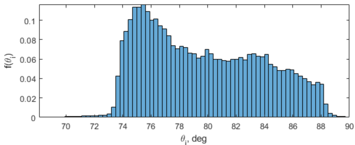
Figure 131: Angular distribution of primary electrons for location 3.
