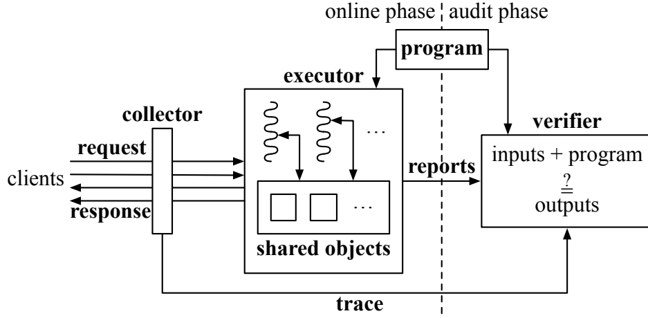
FIGURE 1—The Efficient Server Audit Problem. The objects abstract shared state (databases, key-value stores, memory, etc.). The technical problem is to design the verifier and the reports to enable the verifier, given a trace and a program, to efficiently validate (or invalidate) the contents of responses.
