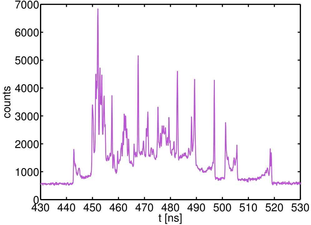
Figure 5-15: Cross-correlation between signal photons detected at LL and idler photons detected on campus for 30 mins with timetagers synced using GPS-based frequency references.
