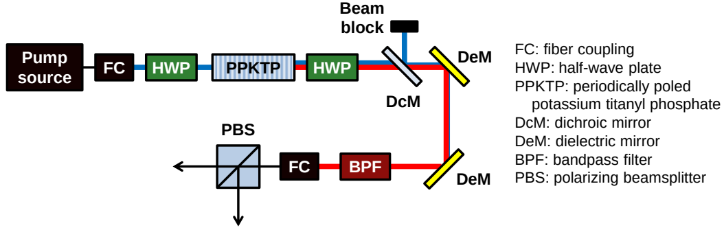
Figure 5-1: Diagram of the campus SPDC source setup. A HWP rotates the pump polarization before the PPKTP waveguide. A second HWP is placed after the waveguide for fine polarization adjustment of the orthogonally polarized signal and idler photons, to maximize the extinction when they are separated by a fiber-based PBS. The pump is extinguished by a combination of dichroic and dielectric mirrors, and the signal and idler photons are coupled into the same PM fiber. Thin, black lines indicate fiber connections; blue lines indicate free-space transmission of the pump beam, and red lines indicate free space transmission of the signal/idler beams.
