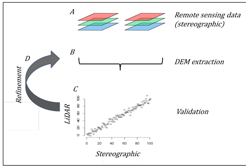
Figure 4. Workflow Diagram.
