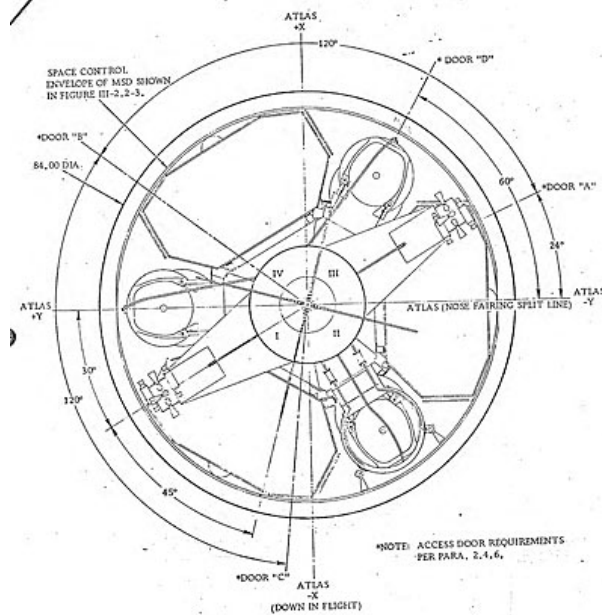
Figure 2. PARCAE Multiple Payload Dispenser Drawing, 1970
