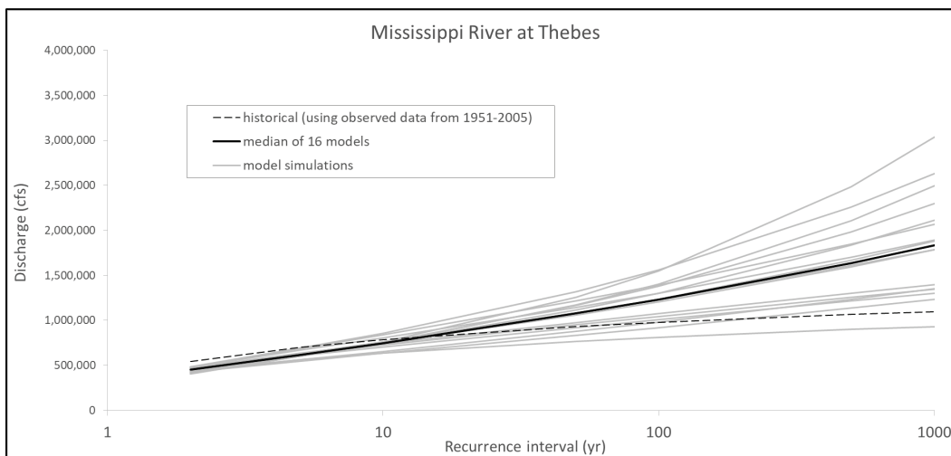
Figure 9. Recurrence interval comparisons for the 1951–2005 time period for the Mississippi River at Thebes, IL.
