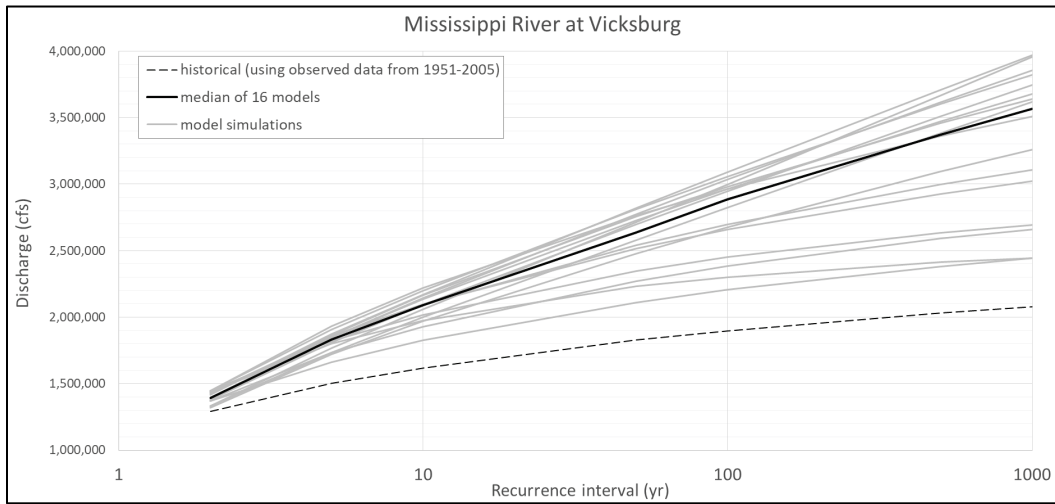
Figure 13. Recurrence interval comparisons for the 1951–2005 time period for the Mississippi River at Vicksburg, MS.
