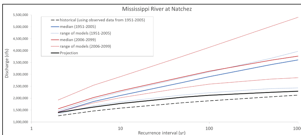
Figure 16. Comparison of recurrence interval changes between the historic and future time periods for the Mississippi River at Natchez, MS.
