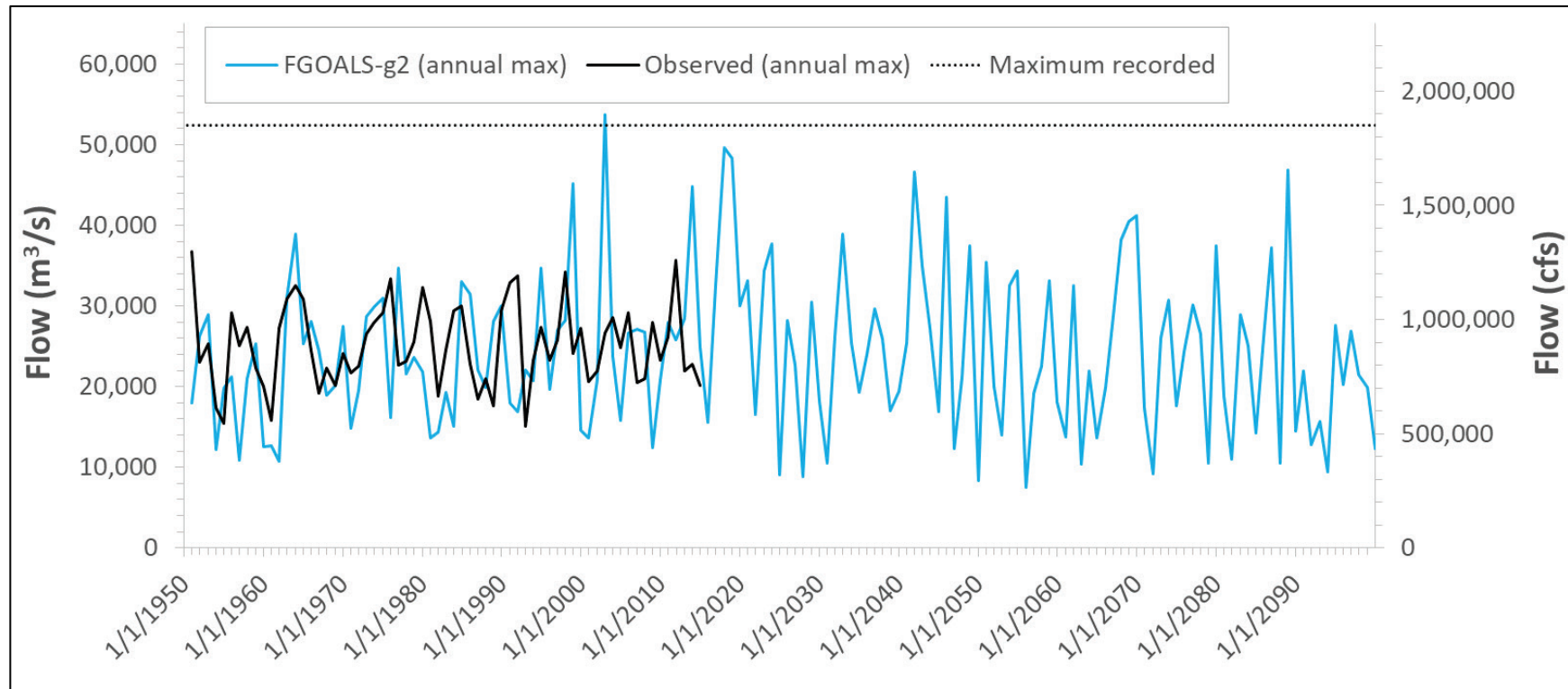
Figure 6. FGOALS-g2 model annual maximum results for the entire simulation time period (1950–2099) for Metropolis, IL.
