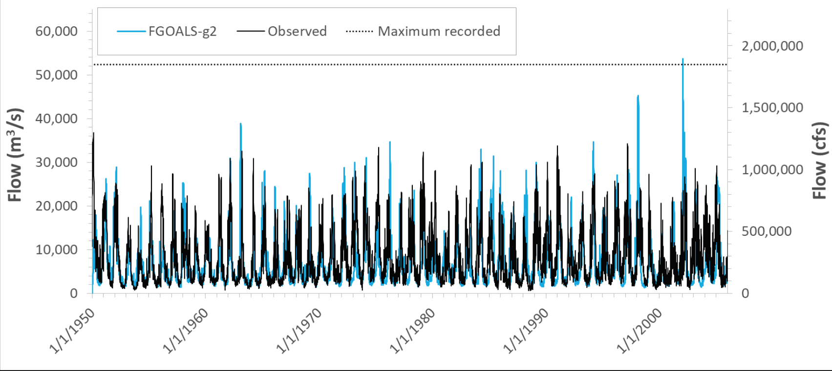
Figure 5. FGOALS-g2 model results for the historical time period (1950–2005) for the Ohio River at Metropolis, IL.
