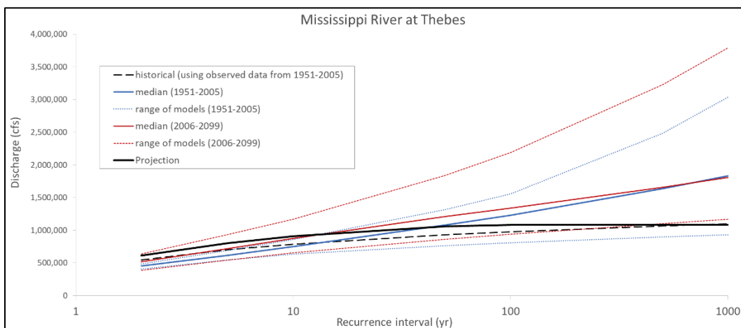
Figure 10. Comparison of recurrence interval changes between the historic and future time periods for the Mississippi River at Thebes, IL.
