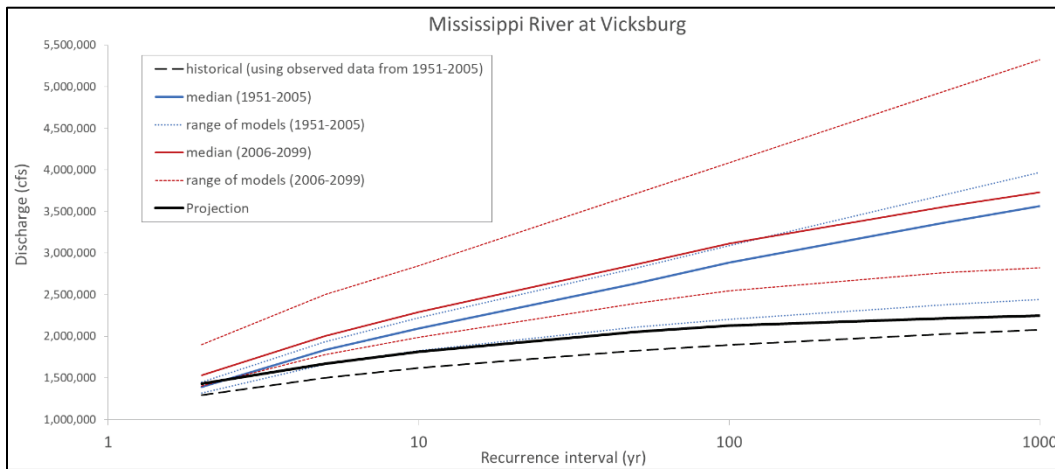
Figure 14. Comparison of recurrence interval changes between the historic and future time periods for the Mississippi River at Vicksburg, MS.
