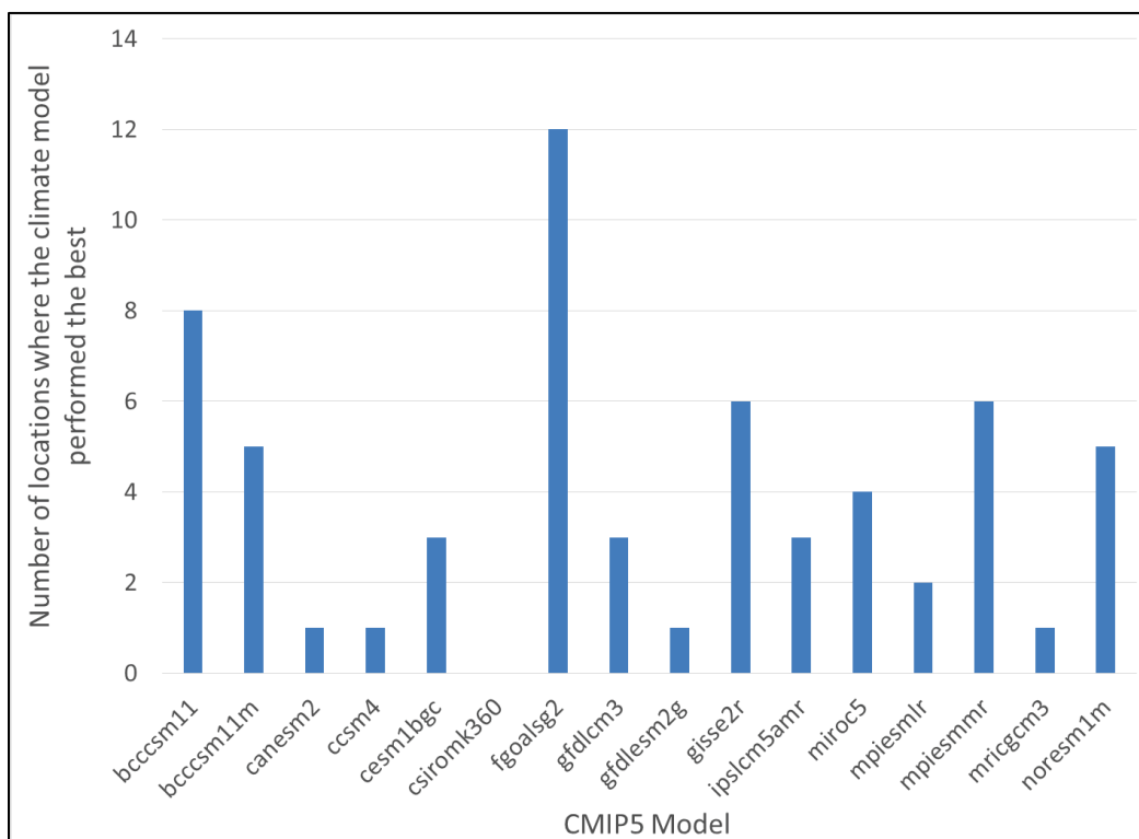
Figure 3. Results of the chi-squared test for all gauges in the study.
