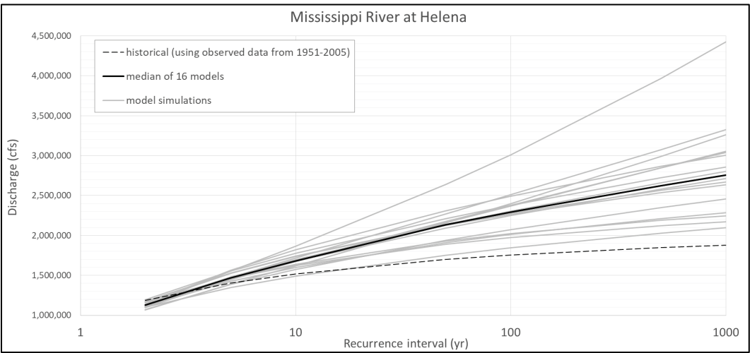
Figure 11. Recurrence interval comparisons for the 1951–2005 time period for the Mississippi River at Helena, AR.
