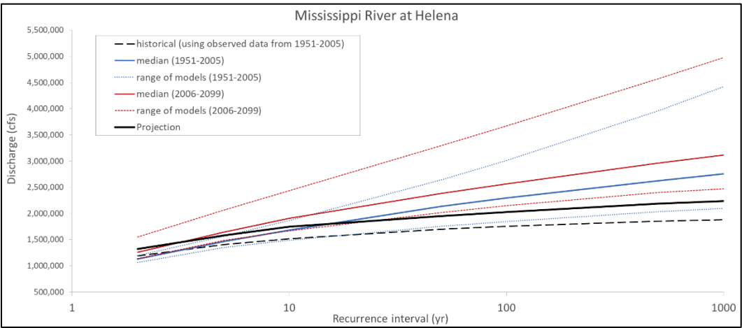
Figure 12. Comparison of recurrence interval changes between the historic and future time periods for the Mississippi River at Helena, AR.
