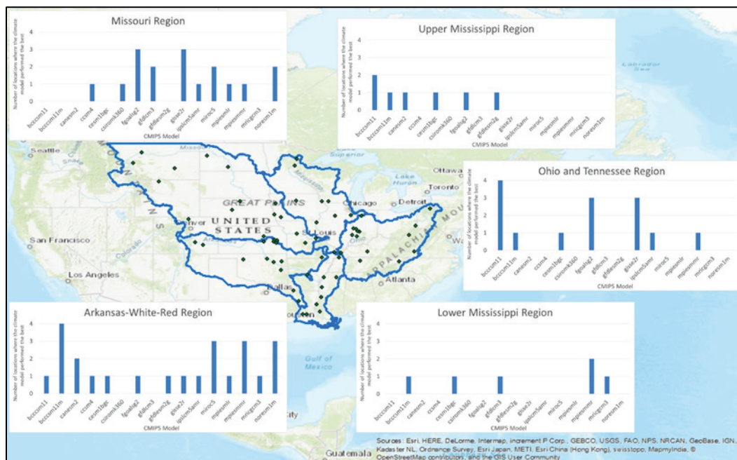
Figure 4. Chi-squared model results by region.
