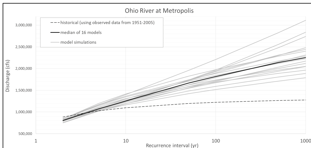
Figure 7. Recurrence interval comparisons for the 1951–2005 time period for the Ohio River at Metropolis, IL.
