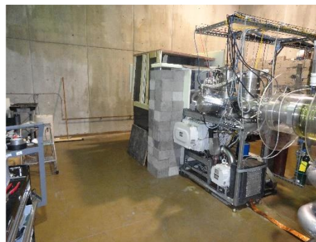
(b) With added graphite, concrete, and boron shielding
