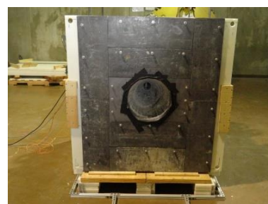
(c) Covered with lead sheeting the to shield image plan
