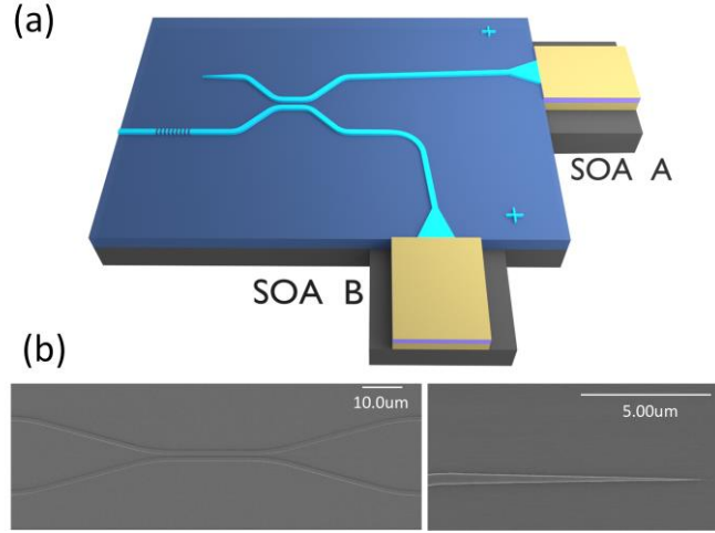
Fig. 4. (a) Schematic plot of the integrated CBC system in the InP- \text{Si}_3\text{N}_4 hybrid platform; (b) Scanning electron microscope images of the fabricated \text{Si}_3\text{N}_4 CBC cavity.
