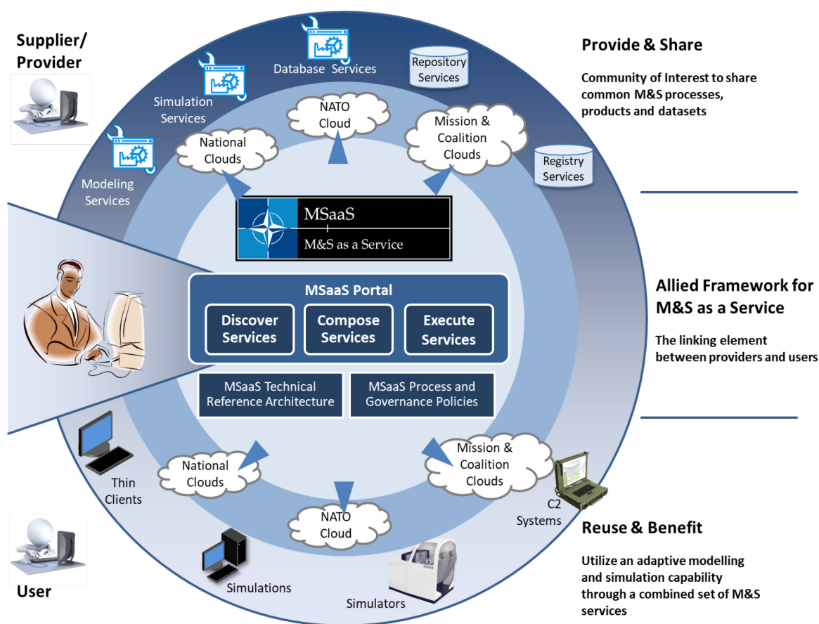
Figure 2-1: Operational Concept of the Allied Framework for M&S as a Service.
