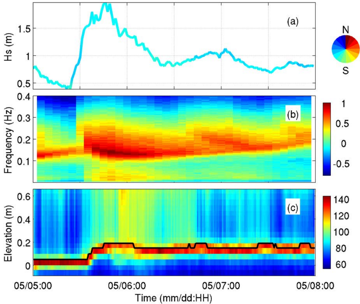
Figure 21. Shown is significant wave height and direction (a) reported as coming from, mean b) free surface spectral density (b) estimated from pressure record, and acoustic backscatter intensity (counts) near the bed (c) with contour of maximum backscatter (solid black line) at the shallow quadpod location.
