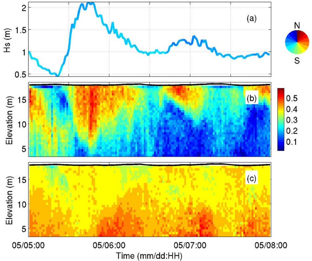
Figure 18. Shown is significant wave height and direction (a) reported as coming from, mean current speed (m/s) and mean surface elevation (solid black line) (b), along with mean current direction (c) reported as flowing towards using same color wheel (a) at the deep quadpod location.
