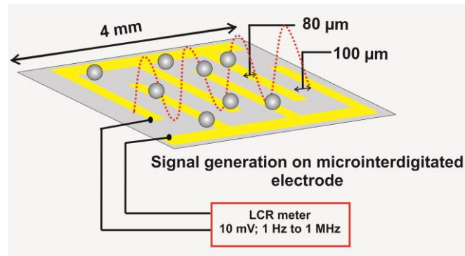
Figure 4. Schematic of the experimental setup used for impedance response measurements of colloidal suspensions. The interdigitated microchip comprised of 80 \mu\text{m} wide finger electrodes with 100 \mu\text{m} edge-to-edge spacing.
