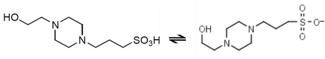
Fig. S8. Molecular structure of EPPS with a single extra carbon atom on the sulfonate side chain as compared to HEPES buffer.
