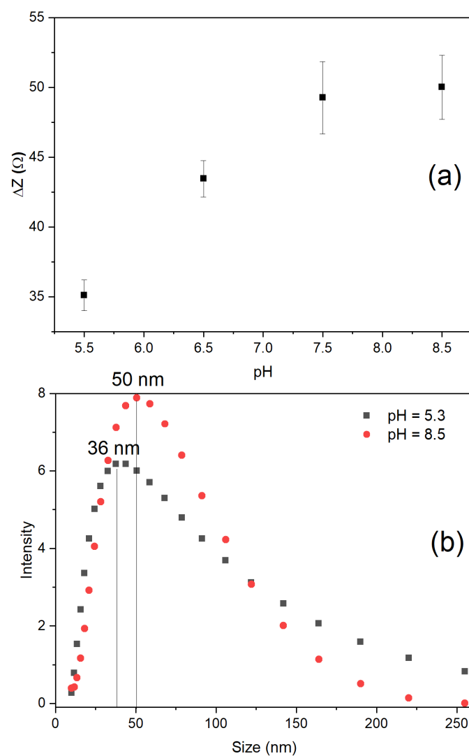
Figure 11. Effect of HEPES buffer pH on the (a) impedance and (b) hydrodynamic diameter of 2% w/v Au NP suspension. The hydrodynamic size of NPs was measured using DLS.
