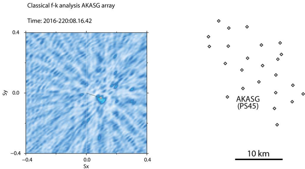
Figure 33. “High-risk” direction estimate of a high frequency signal on a large aperture seismic array (Ukraine example). (left) Slowness estimate for the P_n arrival at the AKASG array (Malin, Ukraine) for an regional earthquake in eastern Ukraine on 7 August 2016. (right) geometry of the AKASG array.
