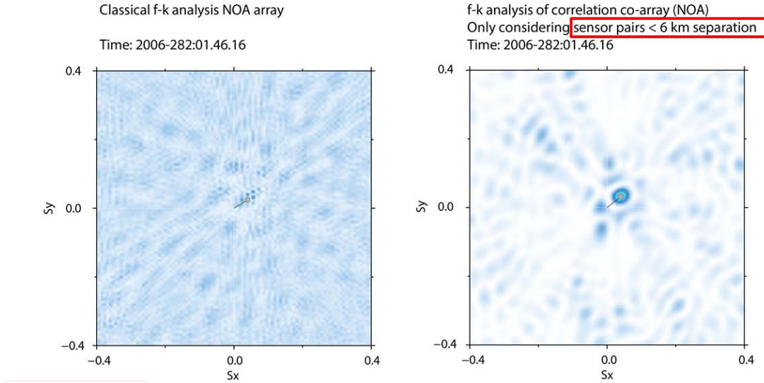
Figure 36. Improvement of direction estimate for the North Korea example using f-k analysis on limited sensor pair correlations. (left) f-k plot from Figure 35 and (right) f-k analysis of correlation co-array containing only sensor pairs with separation below 6 km.
