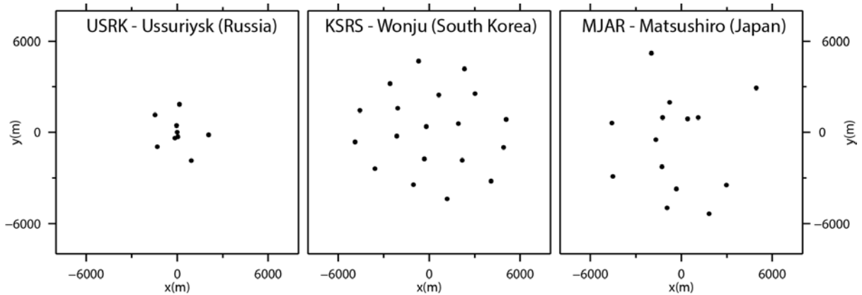
Figure 18. Geometries of the USRK, KSRS, and MJAR seismic arrays. In addition to the differences resulting from the array geometry, there is a significant difference between the degree of waveform similarity observed between sensors of comparable spacing. The KSRS and MJAR arrays have a similar aperture but, due to geologic and topographic factors, wavefronts crossing the MJAR array are far less coherent than those crossing KSRS. Modified from Gibbons and Ringdal (2012).
