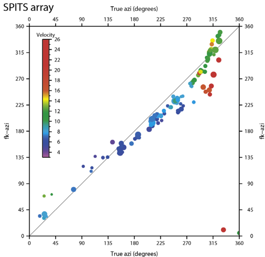
Figure 15. Deviation in backazimuth estimates using classical plane-wave models at SPITS. Variation of the parameter estimates obtained using broadband f - k analysis for the first P -arrival at SPITS as a function of geographical backazimuth obtained using a subset of the Bayesloc locations displayed in Figure 11.
