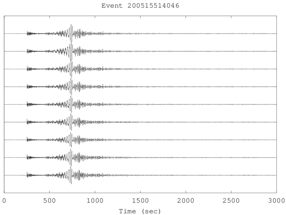
Figure 20. Waveform data for an event in 2005 on day 155 (B line of the Warramunga array only). Surface waves are well recorded at Warramunga for the events shown in Figure 19.
