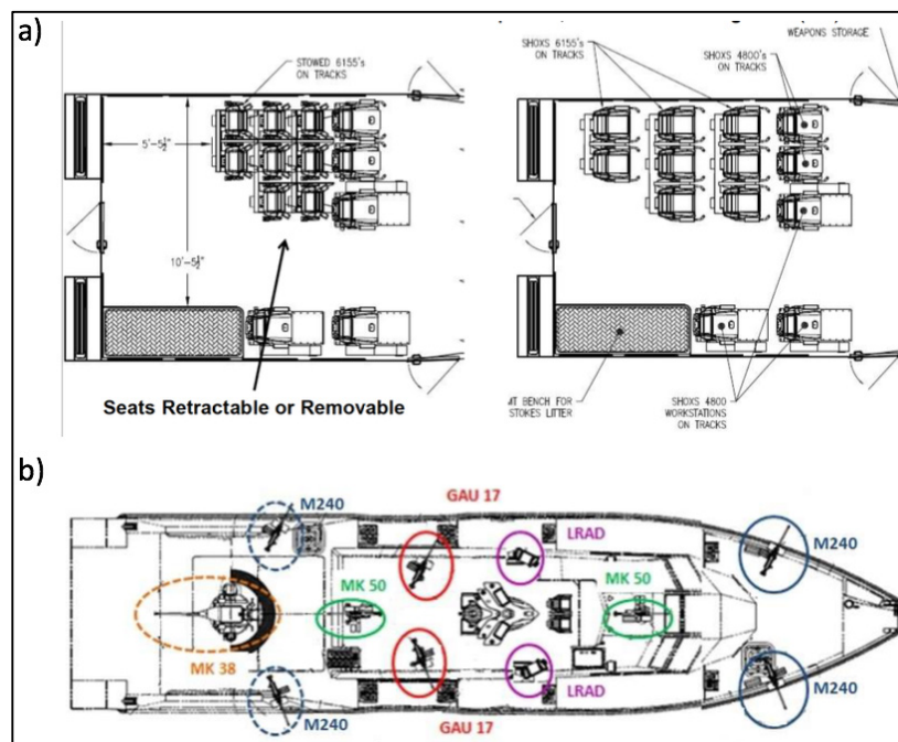
Figure 9. MK VI a) seating and b) weapons configuration. 107
