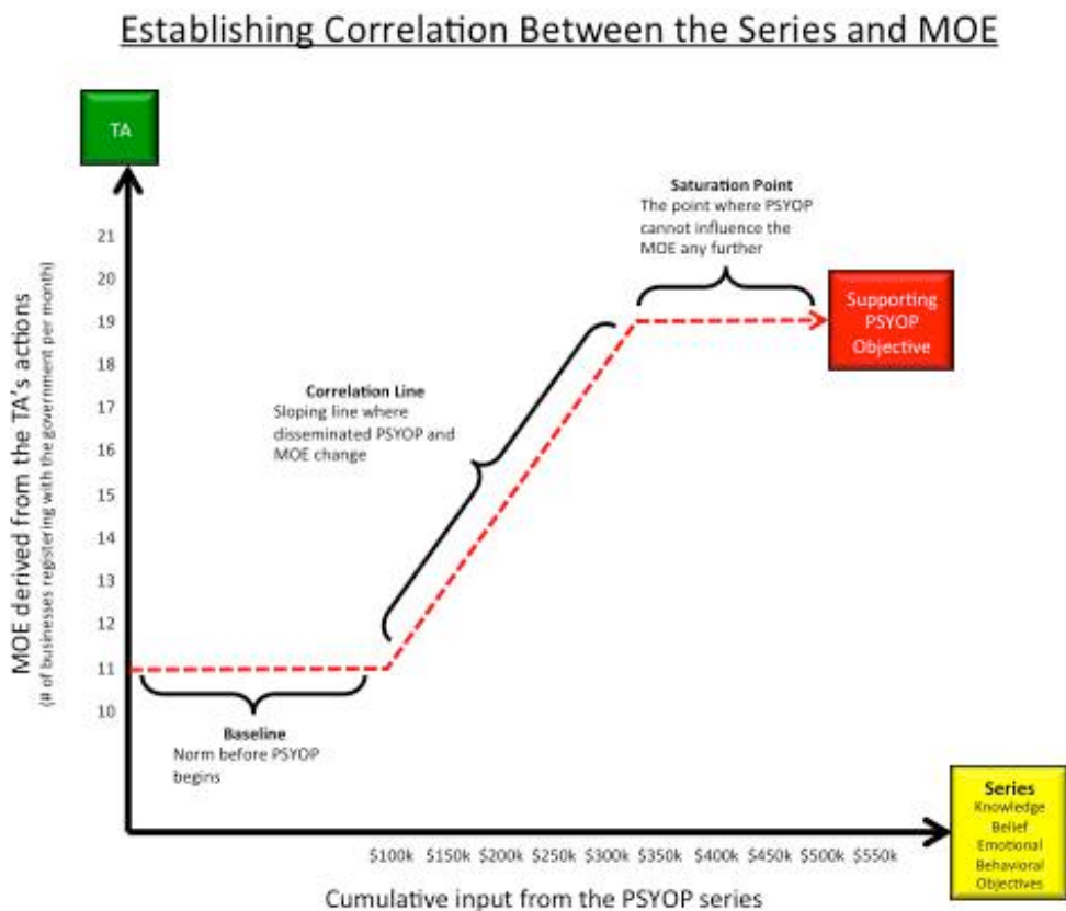
Figure 5. Establishing the Correlation. Between the Series and MOE
