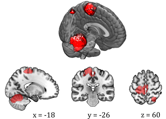
Fig. 3. SDM analyses revealed consistently increased activation in the pre-central gyrus, cerebellum and superior and inferior parietal cortex in response to attempted/imagined movement in patients with spinal cord injury compared to healthy controls.
