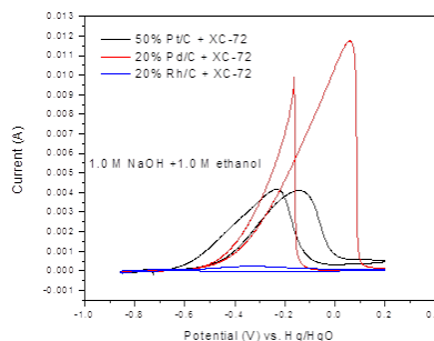
Fig.6. Cyclic voltammogram (CV) curves obtained on anode catalysts (Pt/C, 20% Pd/C and 20% Rh/C) in 1M NaOH and 1M ethanol solutions at room temperature. Scanning rate: 20 \text{ mV sec}^{-1} .
