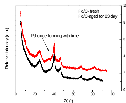
Fig.15. X-ray diffraction spectra obtained with the Pd/C catalyst stored for an extended period.
