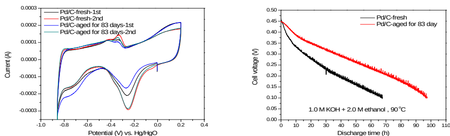
Fig. 16. (a) CV curves obtained with fresh and aged Pd/C catalysts in an Ar-saturated 1.0 M \text{CH}_3\text{CHO} and 1M NaOH solution. Scan rate: 20 \text{ mV sec}^{-1} (b) Stability test by recording cell voltages during discharging direct ethanol fuel cells with fresh or aged Pd/C anode catalysts and circulating 500 mL fuels at constant discharge current density of 100 \text{ mA cm}^{-2} and 90^\circ\text{C} . The fuel contains 2M EtOH and 1M KOH.
