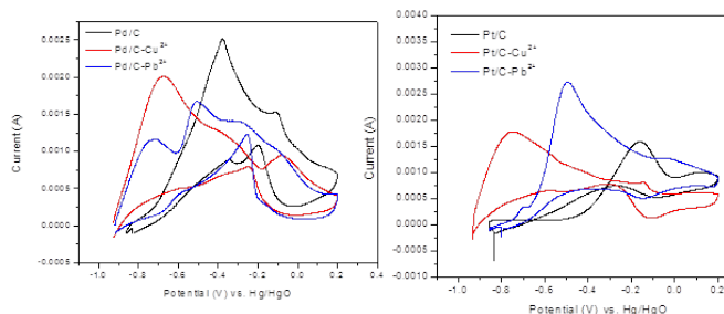
Fig.14. CV curves obtained with (a) Pd/C catalyst and (b) Pt/C catalyst in an Ar-saturated 1.0 M \text{CH}_3\text{CHO} and 1M NaOH solution, or an Ar-saturated 1.0 M \text{CH}_3\text{CHO} and 1.0M NaOH and 1.0 mM \text{CuSO}_4 solution or an Ar-saturated 1.0 M \text{CH}_3\text{CHO} and 1.0M NaOH and 1.0 mM \text{Pb}(\text{CH}_3\text{COO})_2 solution. Scan rate: 20 \text{ mV sec}^{-1}
