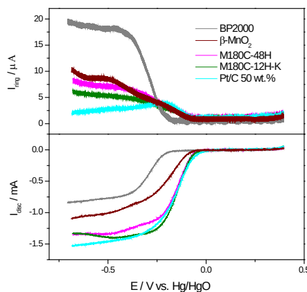
Fig.2. ORR polarization curves of \text{MnO}_2 catalysts with different composition and morphology on a RRDE with a rotation rate of 2500 rpm in \text{O}_2 saturated 0.1 M NaOH. Ring potential E_r = 0.3\text{V} vs. \text{Hg}/\text{HgO} ; Scan rate 10\text{ mV s}^{-1} .
