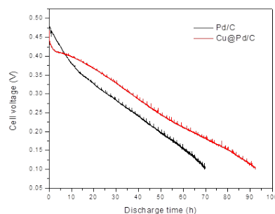
Fig.13. Stability test by recording cell voltages during discharging direct ethanol fuel cells with Pd/C or Cu-modified Pd/C anode catalysts and circulating 500 mL fuels at constant discharge current density of 100 \text{ mA cm}^{-2} and 90^\circ\text{C} . The fuel contains 2M EtOH and 1M KOH.
