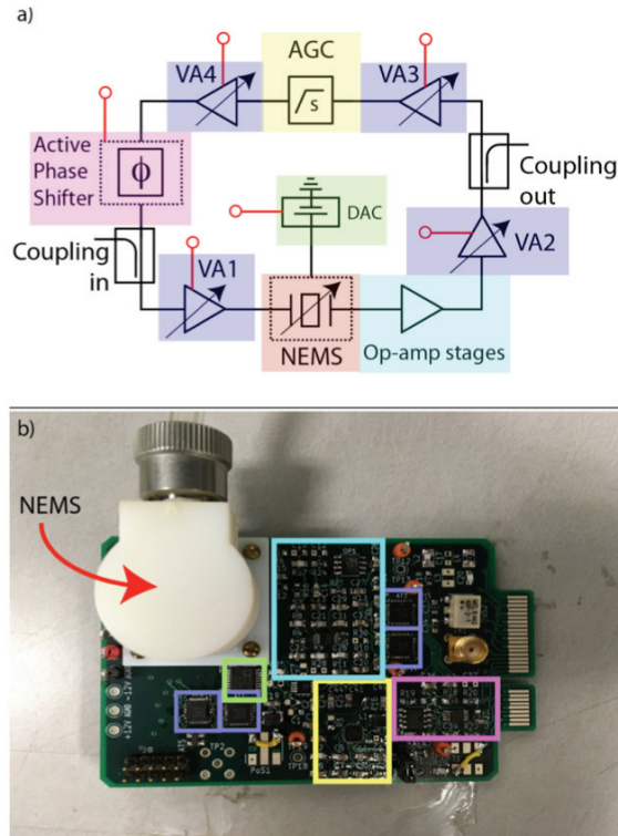
Figure 3: A modular NEMS oscillator node. a) Oscillator board diagram. b) Physical realization of oscillator board (5th gen). The colors in the diagram of a correspond to the color boxes surrounding the components in b).
