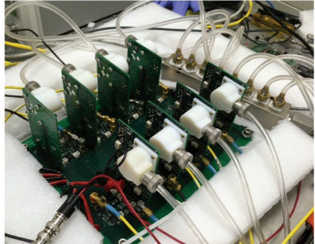
Figure 11: The 8-oscillator NEMS ring network. Note the vacuum manifold on the backside of the ring board (top right), which breaks out the vacuum into 8 separate lines terminating at the individual oscillator modules.
