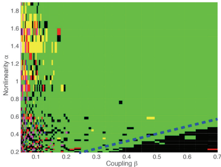
Figure 10: Synchronization diagram for coupling-nonlinearity phase space. Green shows parameter values where only the two splay states are found to be stable. Black is parameter values where all three states are found to be stable. The blue dashed line is the theoretical prediction for the boundary of stability for the fully locked state. Note the black region does not meet this prediction since only 10 experimental trials were taken per point in parameter space.
