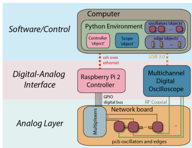
Figure 1: System overview. The system is comprised of three functional layers. The software/controller layer, the digital-analog interface, and the analog layer.
