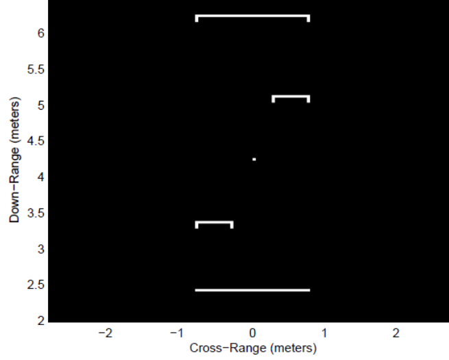
Figure 9. Geometry of the simulated scene.
