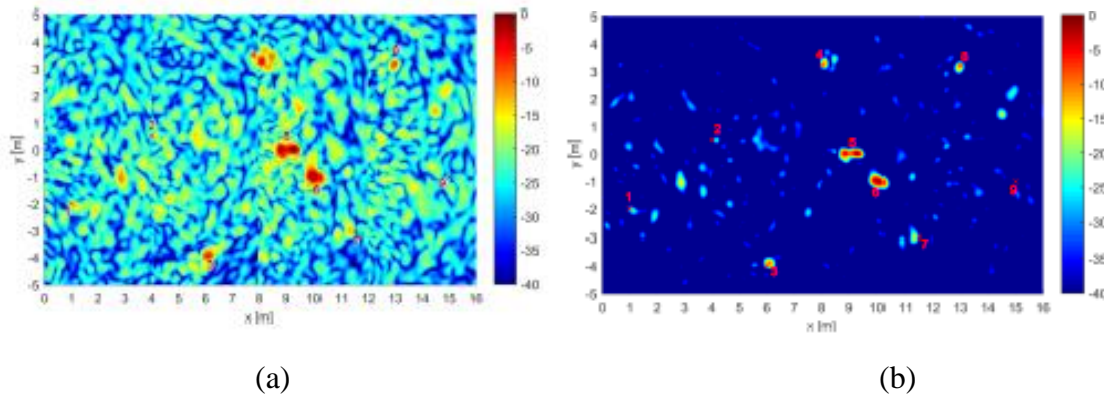
Figure 20. (a) Tomographic image of the ROI. (b) Coherence factor based enhanced image.
