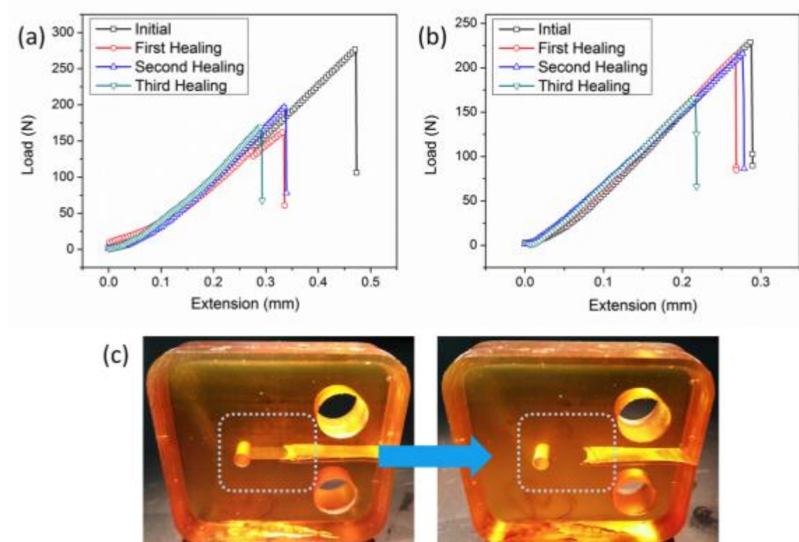
Figure 4. Representative load curves as a function of extension for one, (a) 0.5HTDA1T and (b) 0.8HTDA1T specimen, and (c) one 0.8HTDA1T specimen showing pre- (left) and post-healing (right).
