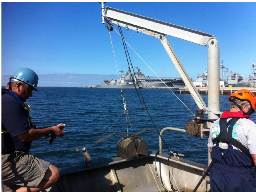
Figure 7. Use of sediment grab to monitor deposition of tracer at the first demonstration site.
