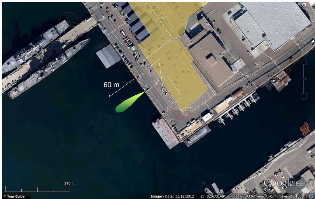
Figure 18. Proposed Outfall 20 location, with drainage basin (top, in yellow), and associated discharge zone plume depicted in the Paleta Creek area south of Pier 8 (bottom, in green).
