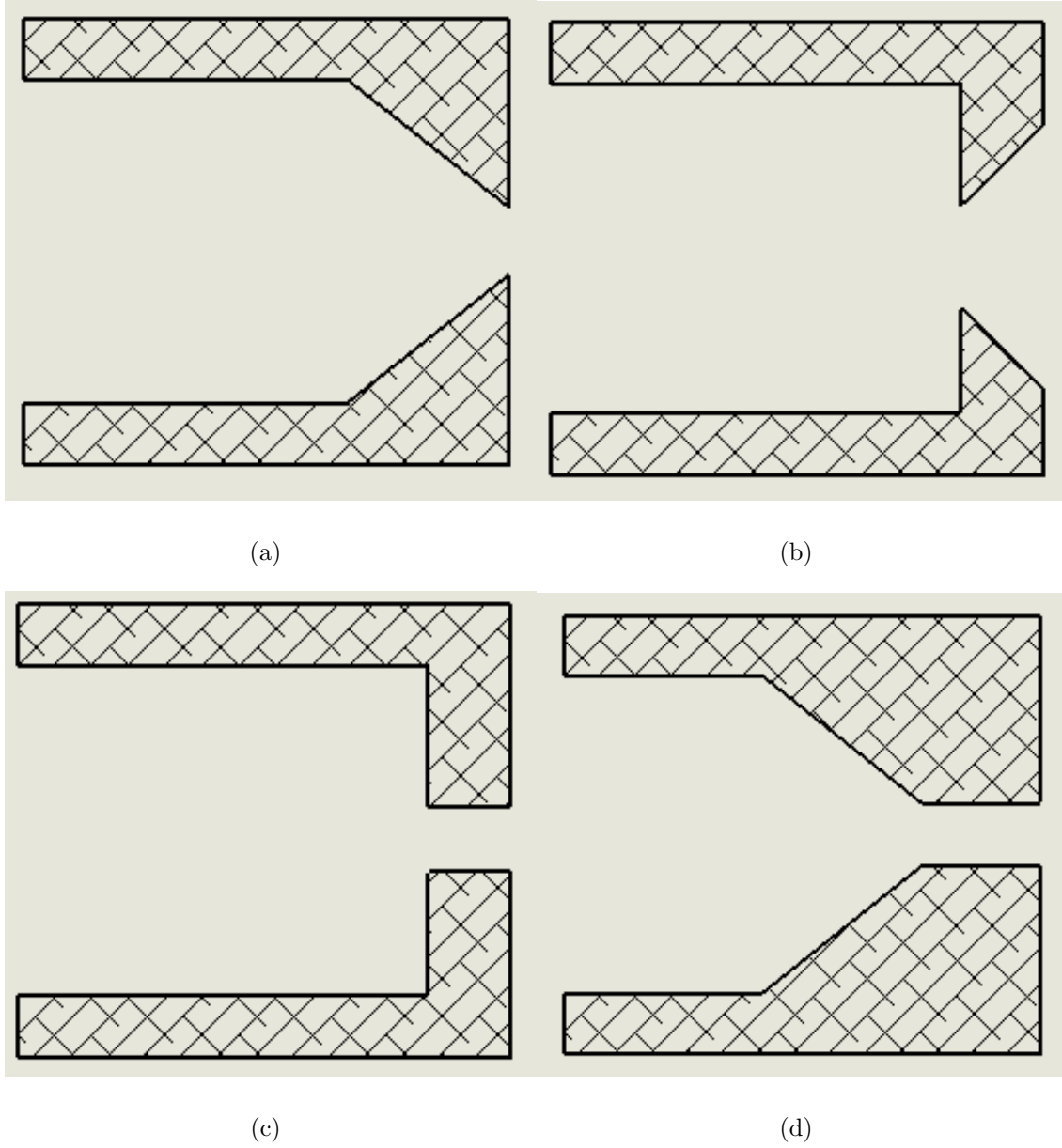
Figure 17. CAD drawings of all four designs, Design 1 (a), Design 2 (b), Design 3 (c), Design 4 (d)
