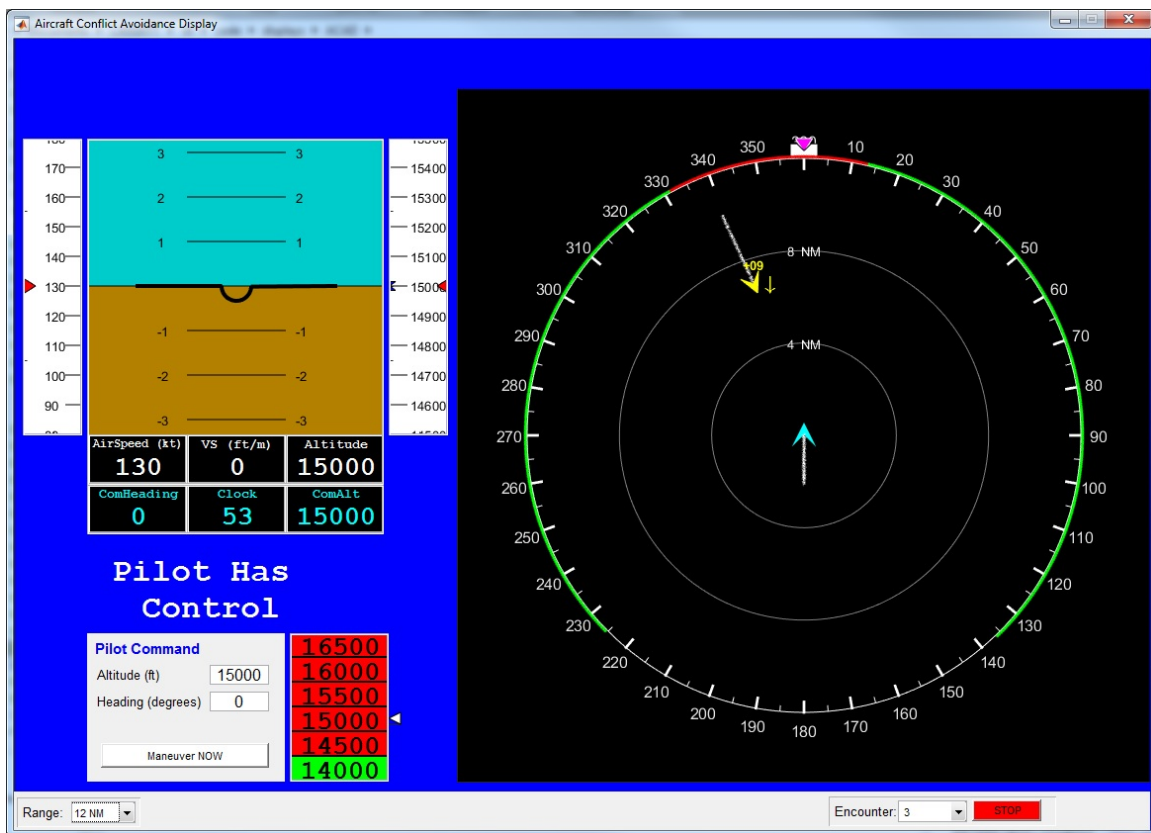
Figure 11. Example of suggestive guidance and associated minimum suggestions.
