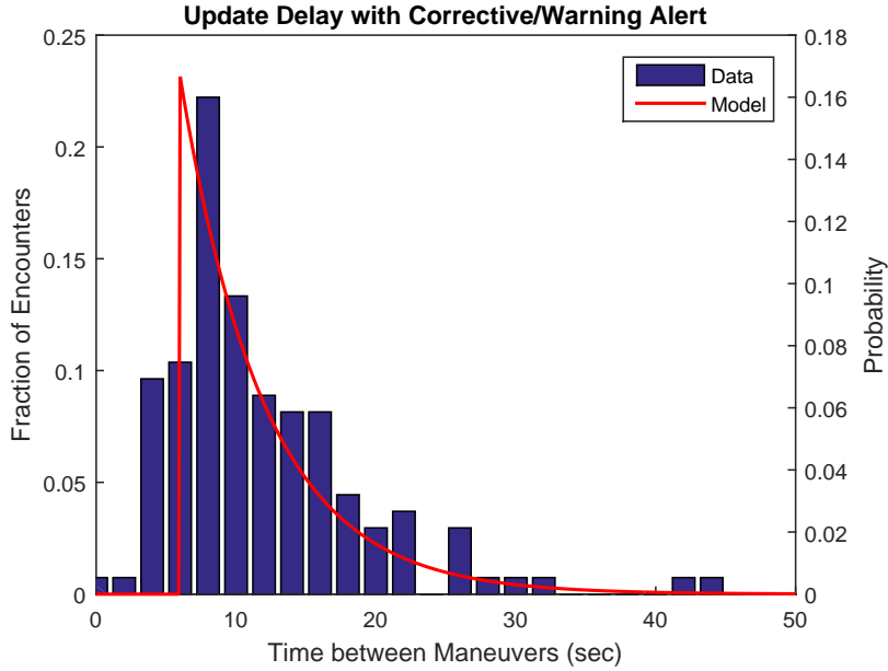
Figure 10. Observed and modeled update delay for corrective or warning alert (Experiment 2 data), shown here with the 3-second average execution delay included.
