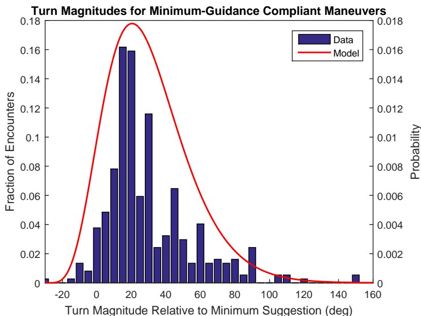
Figure 13. Observed and modeled turn magnitudes for minimum-guidance compliant maneuvers (Experiment 2 data).
