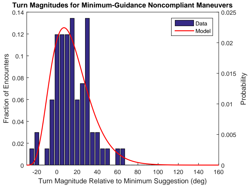
Figure 14. Observed and modeled turn magnitudes for maneuvers not following minimum guidance (Experiment 2 data).
