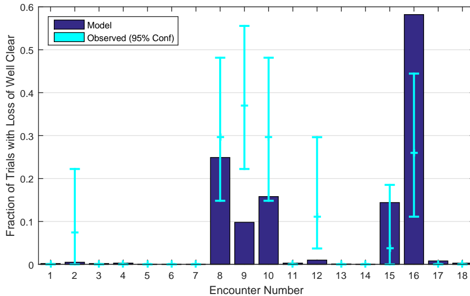
Figure 17. Comparison of observed and simulated losses of well clear.
