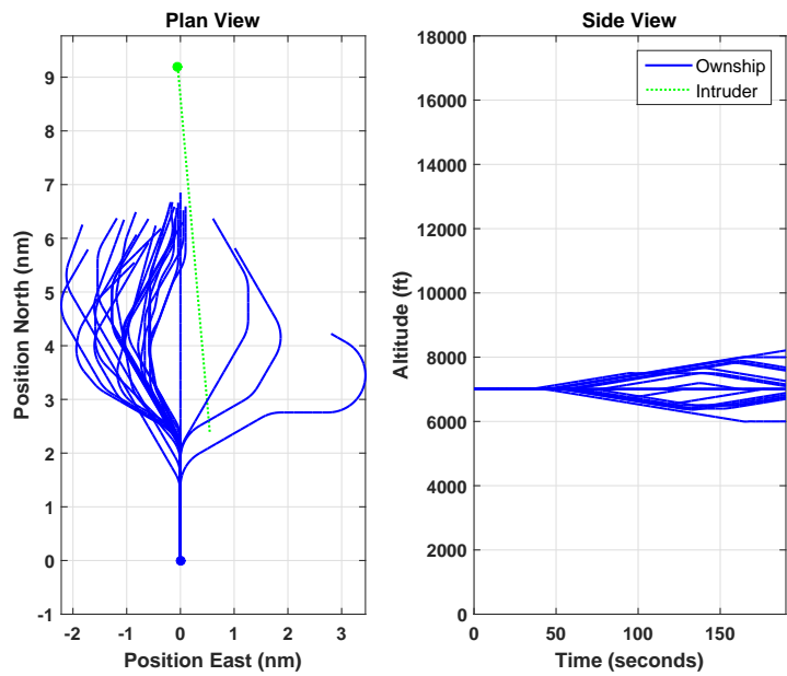
Figure 4. All pilot responses for encounter 1 in Experiment 2.
