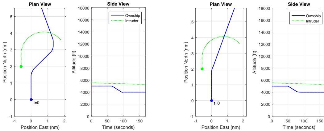
Figure 16. One response observed in Experiment 2 (left) and a simulated response (right).
