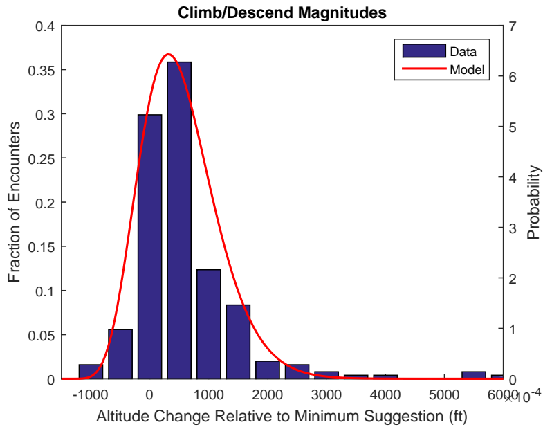
Figure 15. Observed and modeled climb/descend magnitudes for all vertical maneuvers (Experiment 2 data).
