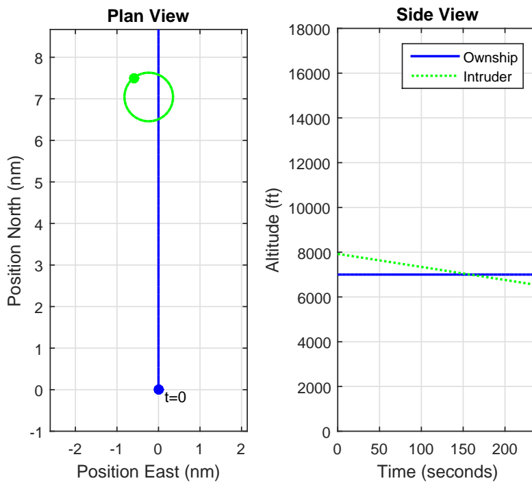
Figure 20. Experiment 2 encounter #16 trajectories.
