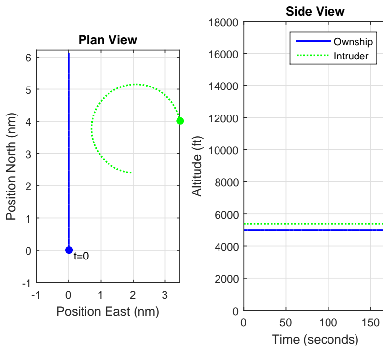
Figure 18. Experiment 2 encounter #9 trajectories.
