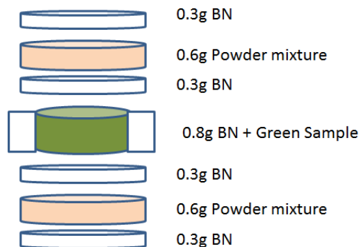
Figure 3.4 – Schematic showing the powder bed used for hot pressing \alpha' -SiAlON samples.
