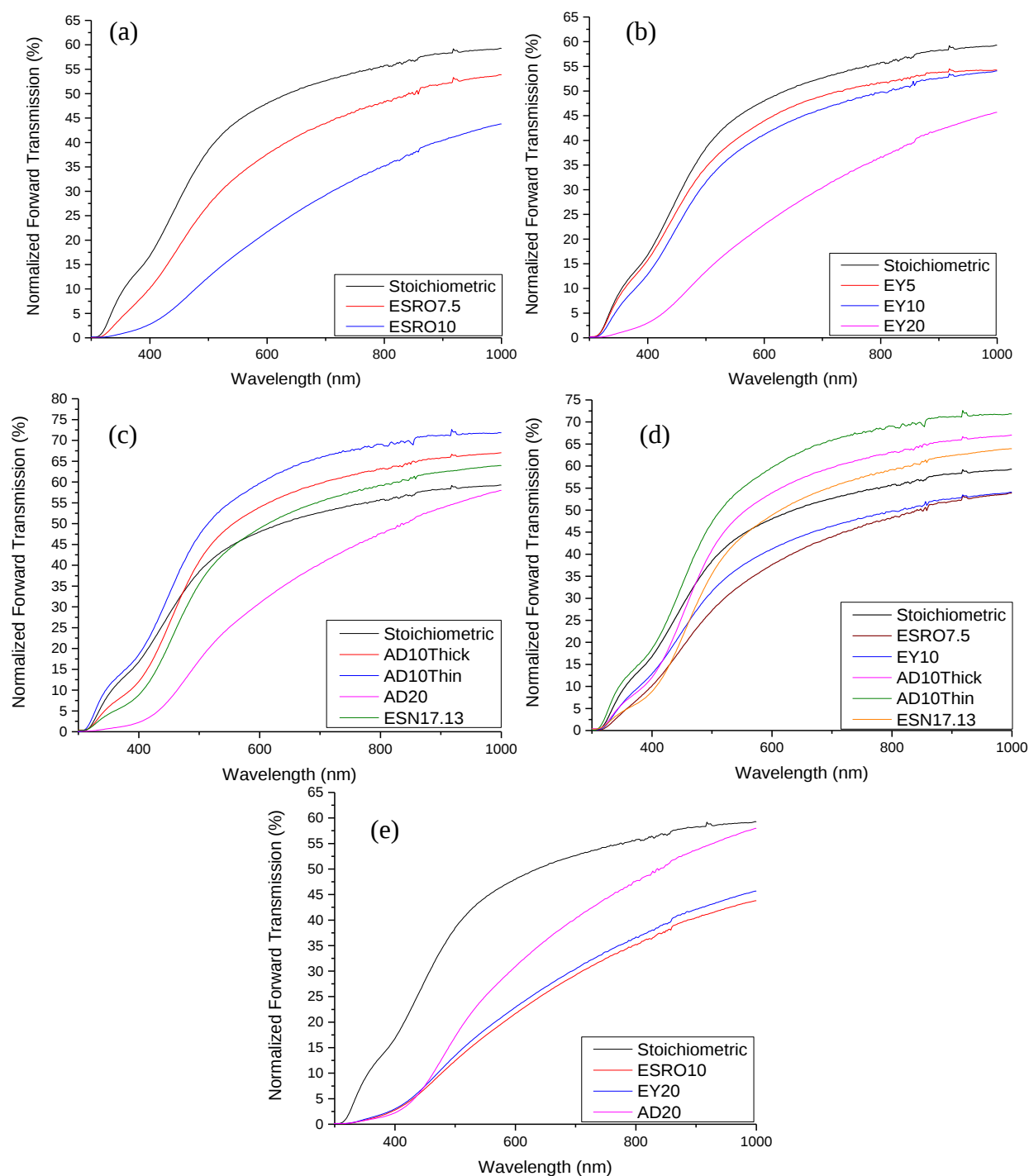
Figure 3.18– UV-Visible Transmission data for each sample series compared to the stoichiometric sample. (a) ERSO7.5 and ERSO10 samples. (b) EY5, EY10, and EY20 samples. (c) AD10Thick, AD10Thin, AD20, and ESN17.13 samples. (d) Compares the compositions with the best transmission from each composition series. (e) Compares the end member samples. All data was normalized to the thickness of the samples using eq. 3.5.
