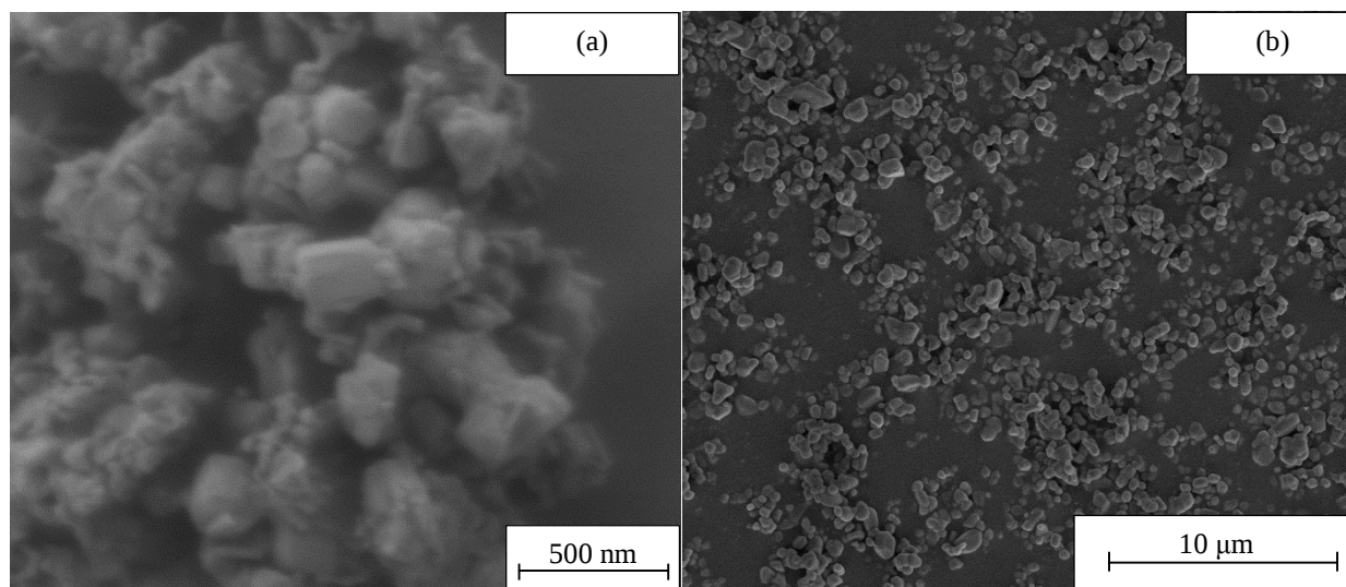
Figure 3.3 - SEM micrographs of the as-received Si 3 N 4 and AlN powders, respectively.
