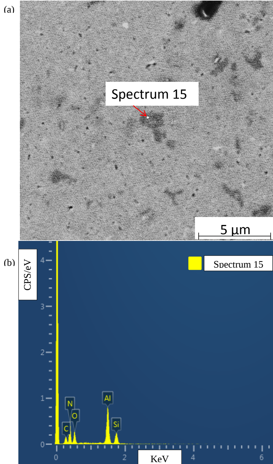
Figure 3.6 – (a) BSE image of ESRO10 showing the location of spot EDS analysis on the dark phase. The white dots in the middle of the micrograph show where the EDS analysis was done. (b) Showing the EDS spectra from the spot analysis. Similar EDS spectra were seen in all samples containing AlN-polytypoids. The accelerating voltage was 5 keV. The interrogated volume is approximately 0.014 \mu\text{m}^3 .
