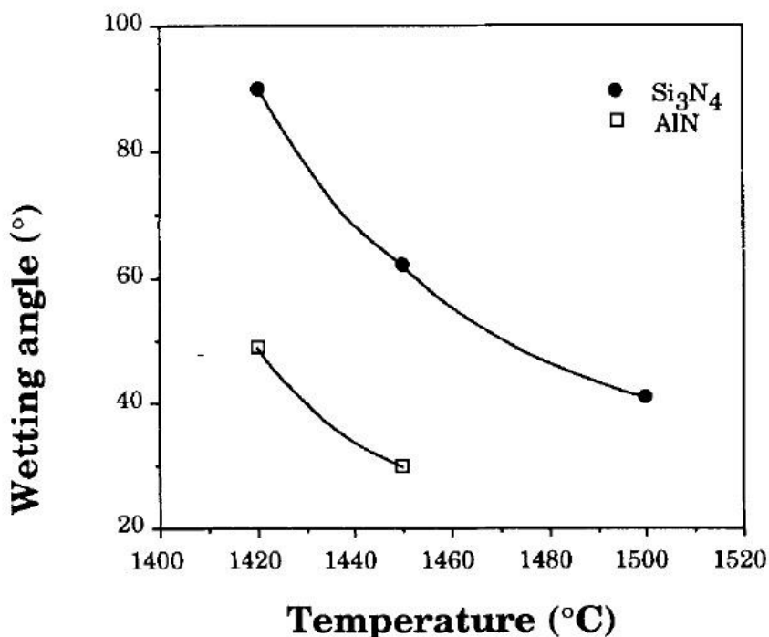
Figure 2.9 – Wetting angle variation vs temperature of the Y_2O_3 - Al_2O_3 - SiO_2 eutectic oxide on AlN and Si_3N_4 substrates. Only two data points are shown for the AlN substrate because the melt completely reacted with substrate at the final measuring temperature. 70
