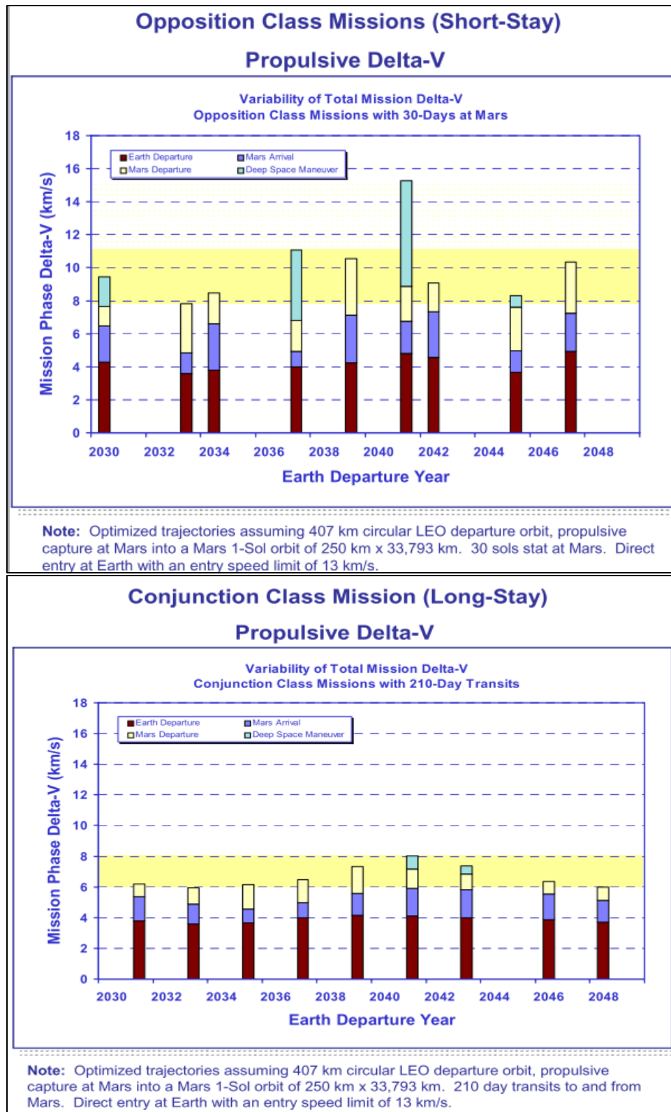
Figure 34. Delta V Comparisons. Source: Drake (2009, 57).
