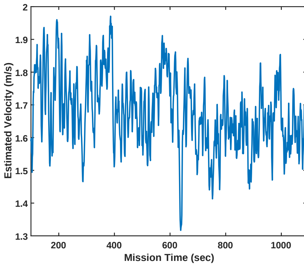
Figure 4.5. REMUS Estimated Forward Velocity
