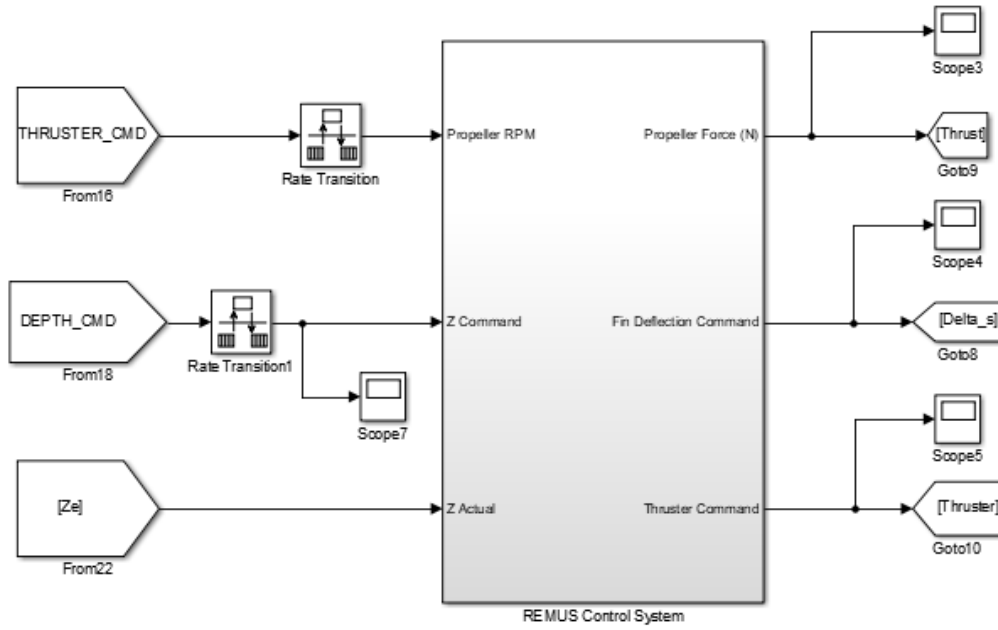
Figure 3.5. Controller Importing Real World Commands.
