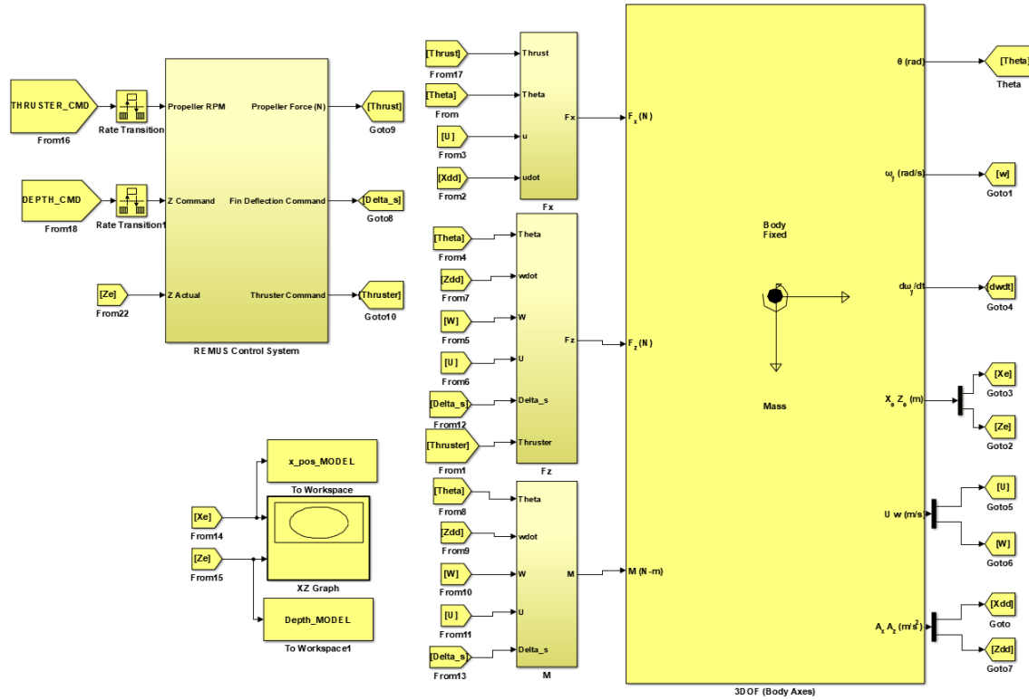
Figure 3.6. Complete Variable Speed REMUS Model Utilizing Cross-Tunnel Thrusters.
