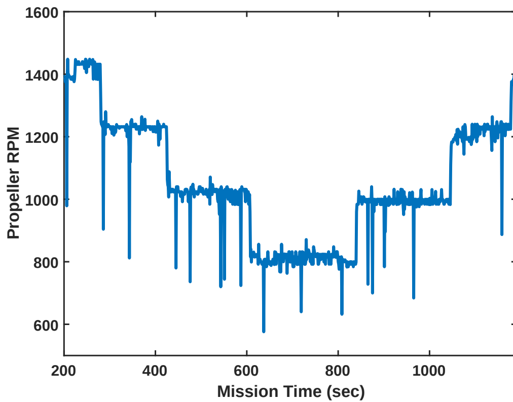
Figure 4.2. Real World RPM Commands
