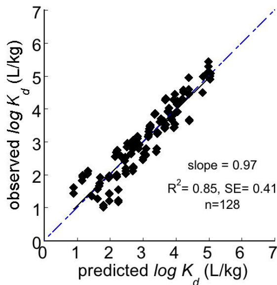
Figure 6. Overall correlation of the individual observed sorption coefficients with the ppLFER predicted sorption coefficients on chestnut wood char.
