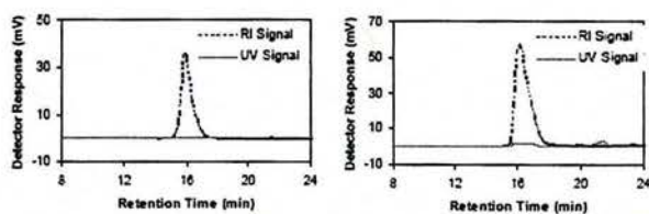
Figure 2.6. GPC traces before (left) and after (right) LFP 7 was subjected to the testing conditions, except ultrasound was omitted. LFP 7 was dissolved in acetonitrile (0.75 mg/mL) containing N-pyrene maleimide trap (2.75 mg/mL, ca 500 equiv), purged with argon and cooled to ca 1 °C. After standing for 45 min, the solvent was removed and the polymer was purified by preparatory GPC.
