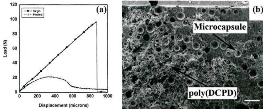
Figure 1.9. a. In-situ mechanical response of a sample containing 12 wt% recrystallized \text{WCl}_6 and 15 wt% 188 \pm 31 \mu\text{m} capsules and b. SEM image of the fracture surface of an in-situ sample after healing and refracture. [scale bar = 500 \mu\text{m} ]
