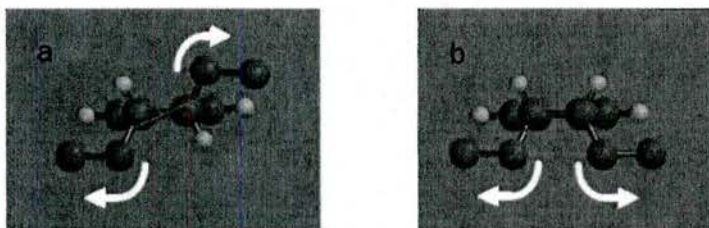
Figure 2.3. The difference between the efficiency of stress activation between trans and cis benzocyclobutene has been attributed to effective torque. a) In trans -benzocyclobutenes, elongational stress applied along the red vector induces a conrotatory motion of the substituents to yield an E,E- o QDM intermediate. b) In cis -benzocyclobutenes, elongational stress applied along the red vector induces a disrotatory motion of the substituents, leading to an E,E- o QDM intermediate.
