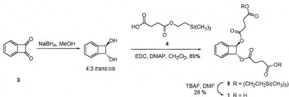
Scheme 2.1. Preparation of trans -benzocyclobutene linker 1 .
