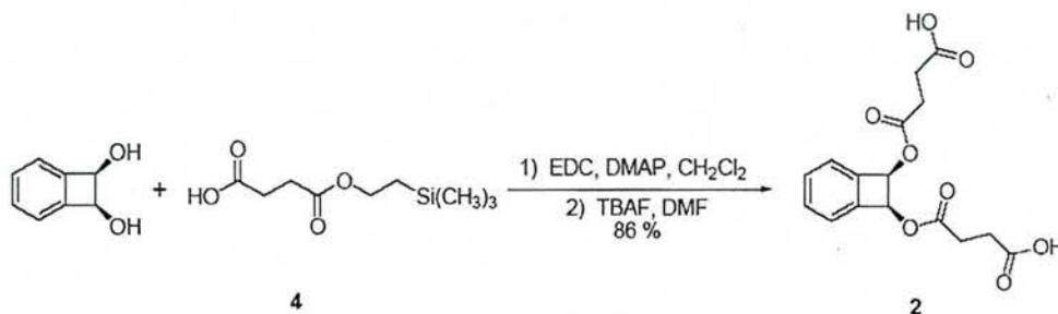
Scheme 2.2. Preparation of cis -benzocyclobutene linker 2 .
