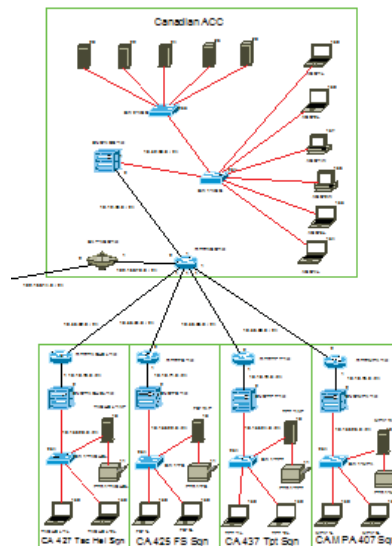
Figure 12: CWID IT Infrastructure for Deployed Air
