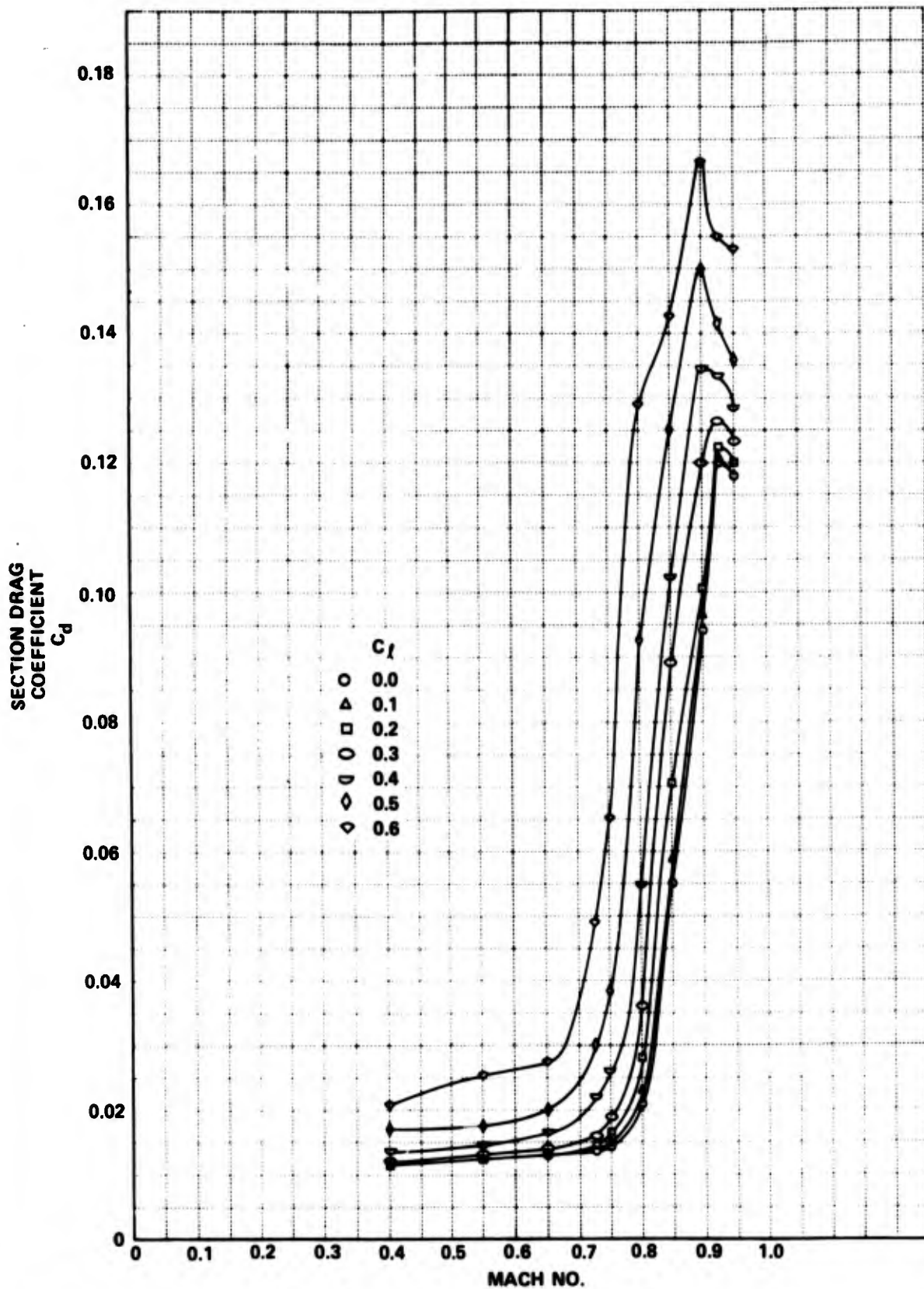
Figure 8 AIRFOIL DRAG COEFFICIENT, Re = 10^6
