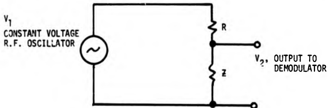
Figure 2. Basic Sensing Concept
