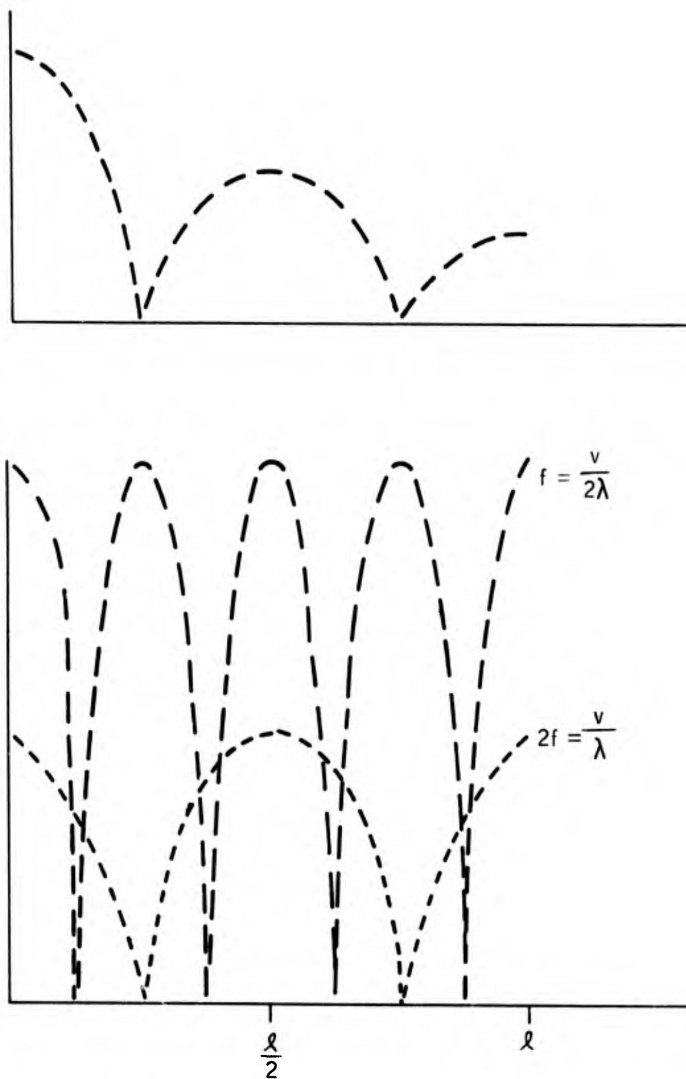
Figure 29. Ideal Standing Wave Pattern Sensitivity at \lambda and 2\lambda Drive Frequencies
