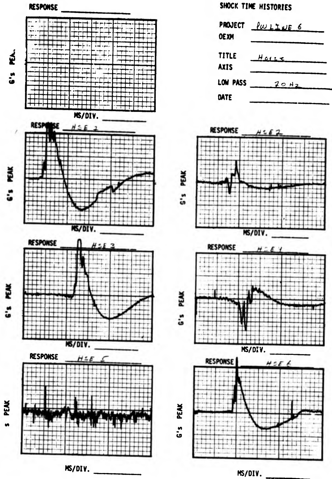
Figure 39. First HOPG Data from 260 Feet (80-Meter Line) (Concluded)
