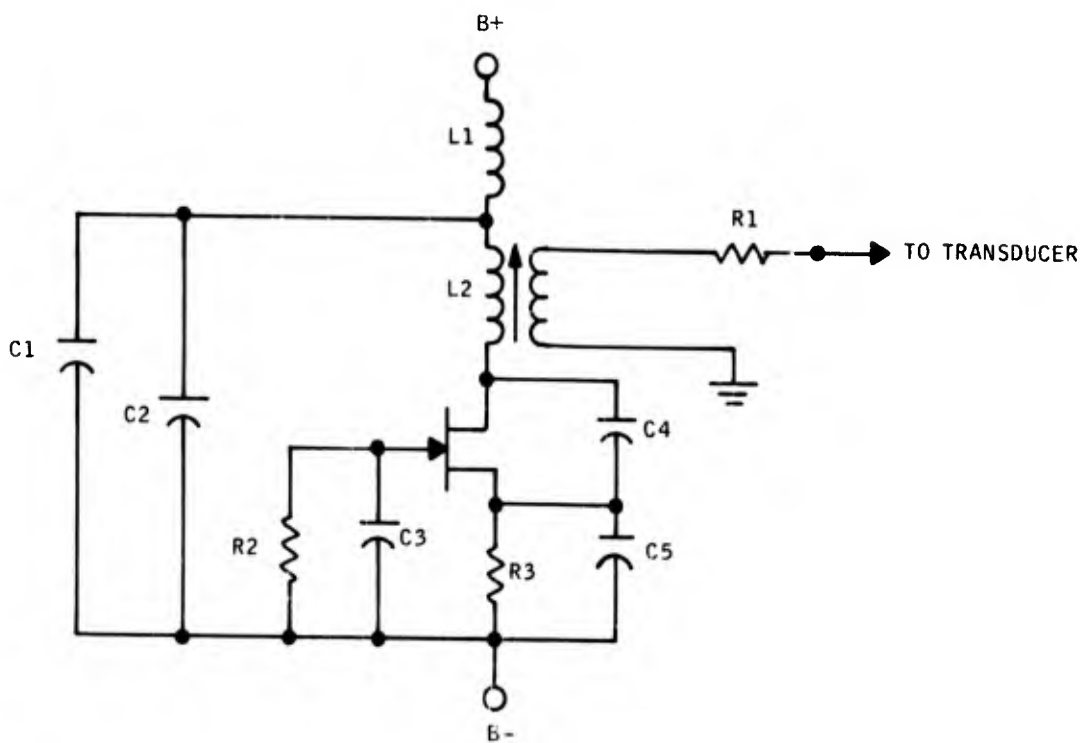
Figure 14. Oscillator/Line Driver Schematic
