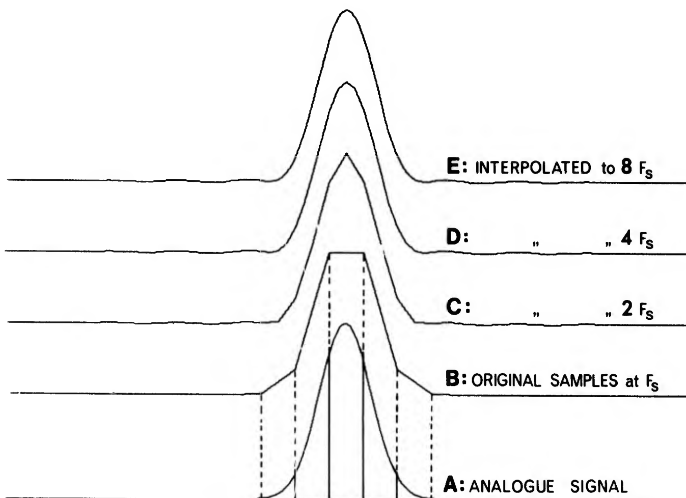
FIG. 6 INTERPOLATION OF A SAMPLED GAUSSIAN PULSE \exp[-\frac{1}{2}(t/\tau)^2] Original sampling frequency F_s = 0.8/\tau (4 times the 6 dB cut-off frequency)
