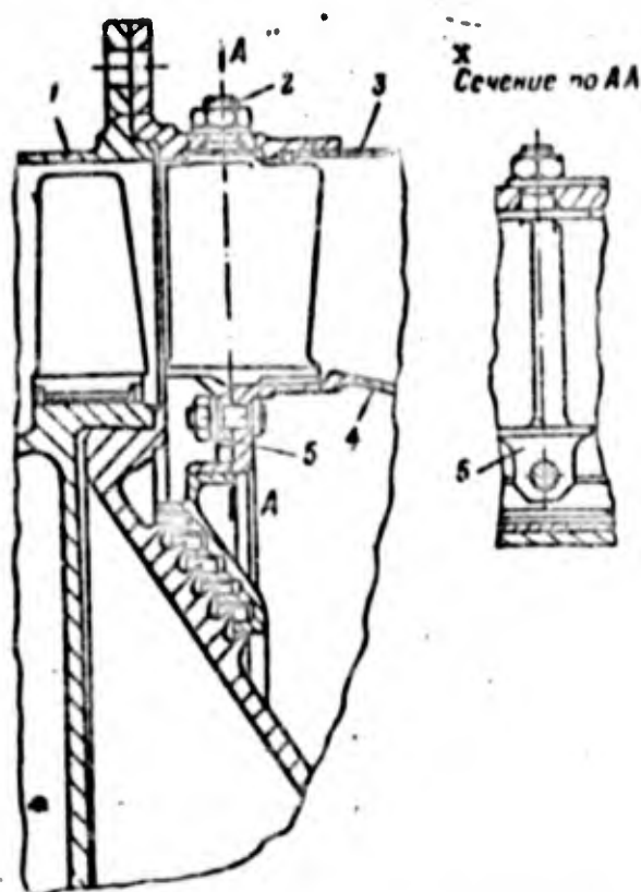
Fig. 46. Stator vane assembly of the last compressor stage. 1) Compressor casing; 2) journal; 3) outer casing of the combustion chamber; 4) inner casing of the combustion chamber; 5) lug. x) Section through A.A.
