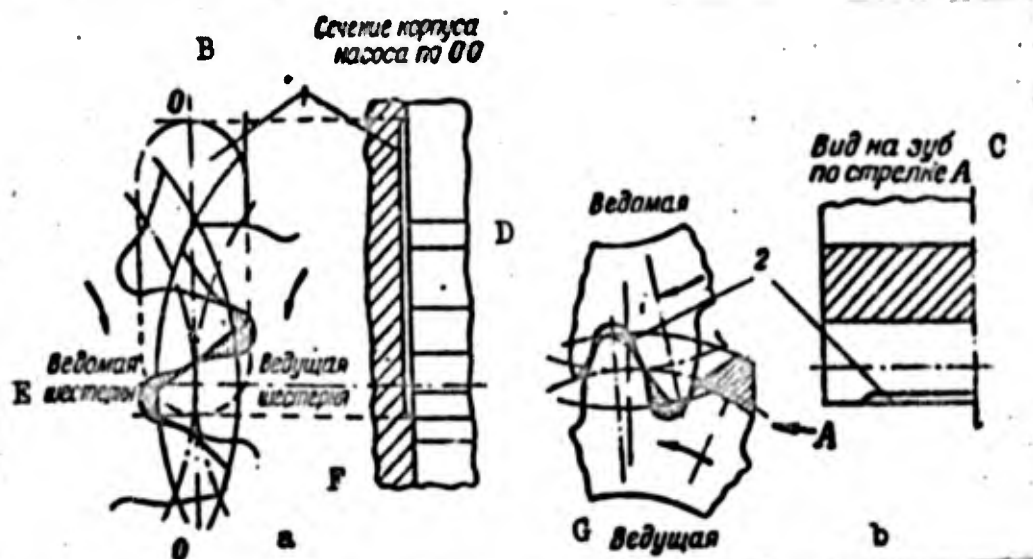
Fig. 170. Relief grooves. a) In the pump housing; b) on the nonworking sides of the teeth; 1 and 2) grooves; B) cross-section of pump housing along 00; C) view toward tooth along arrow A; D) driven; E) driven gear; F) driving gear; G) driving.
