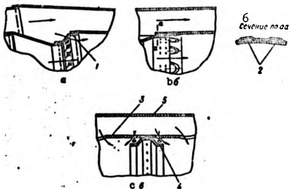
Fig. 108. Methods of supplying cooling air for boundary-layer cooling: 1) ring with vents; 2) slots; 3) duct; 4) shaped ring; 5) housing; 6) section through aa.
