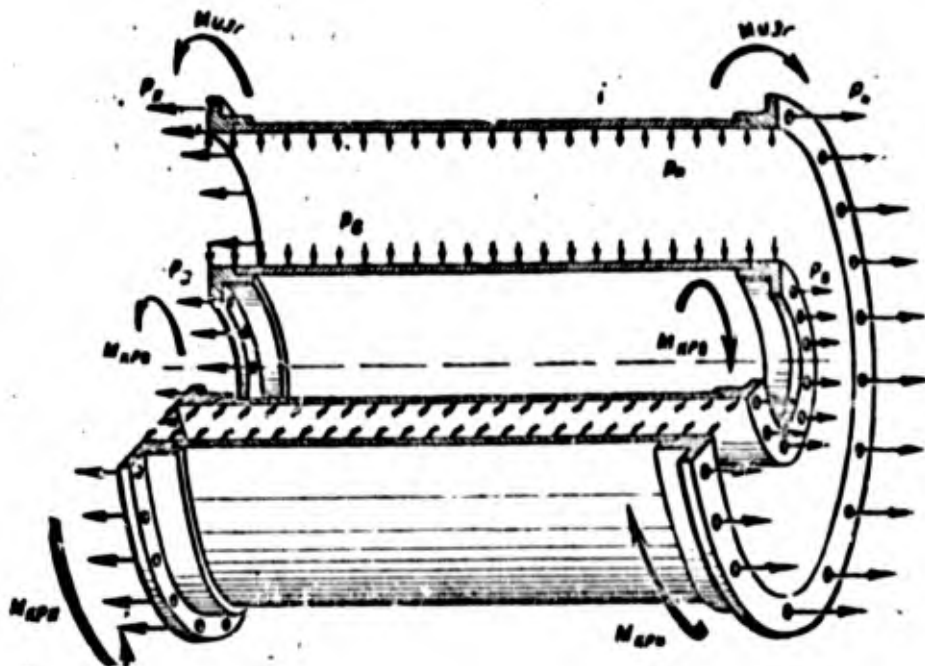
Fig. 113. Loading of outside and inside rings of annular and cannular combustion chambers.
