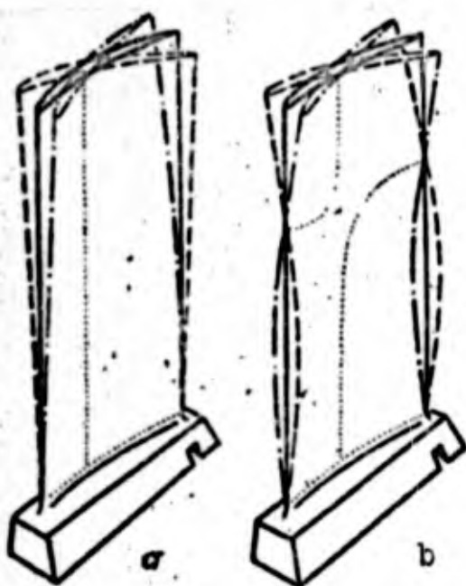
Fig. 23. Modes of torsional blade vibration. a) First; and b) second.
