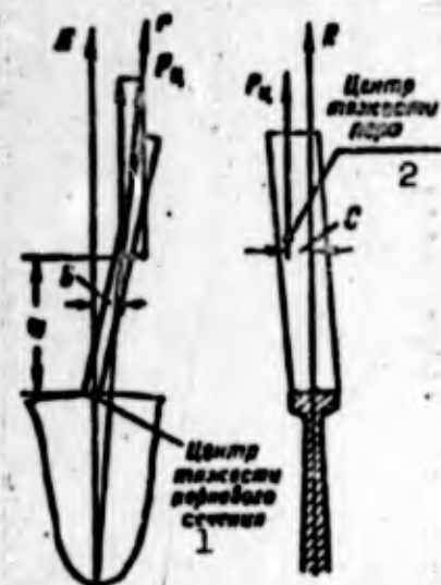
Fig. 20. Compensation of the bending of a blade by use of the moment due to centrifugal forces. 1) Center of gravity of root section; 2) center of gravity of the fin.
