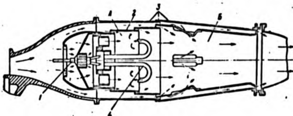
Fig. 99. Straight-through flow combustion chamber with fuel supplied as the vapor: A) combustion zone; B) mixing zone; 1) nozzle; 2) flame tube; 3) chamber housing; 4) vaporization tube (for vaporized-fuel injector, see Fig. 208).
