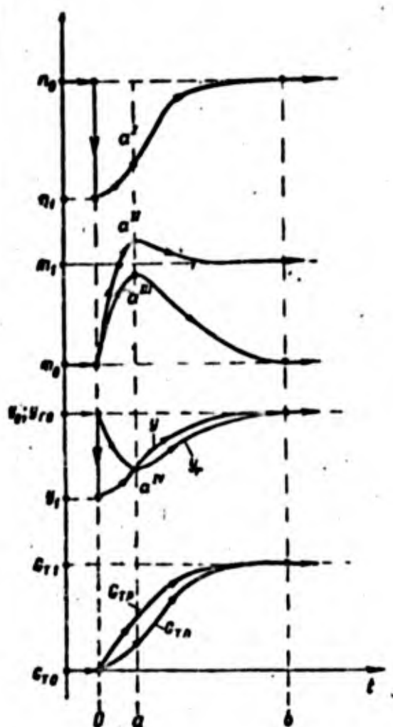
Fig. 261. Motion of control system with proportional-plus-integral feedback during transient.
