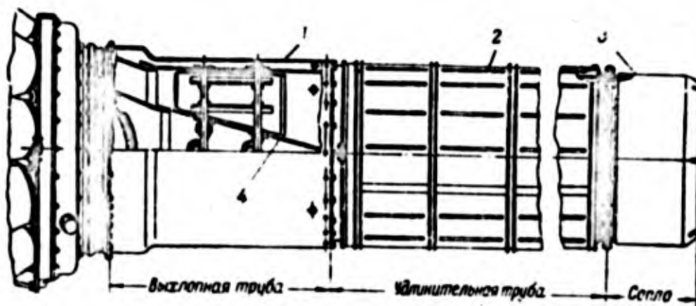
Fig. 116. Exhaust section for TRD [turbojet engine]: 1) exhaust pipe; 2) extension pipe; 3) nozzle; 4) inside cone; 5) exhaust pipe; 6) extension pipe; 7) nozzle.
