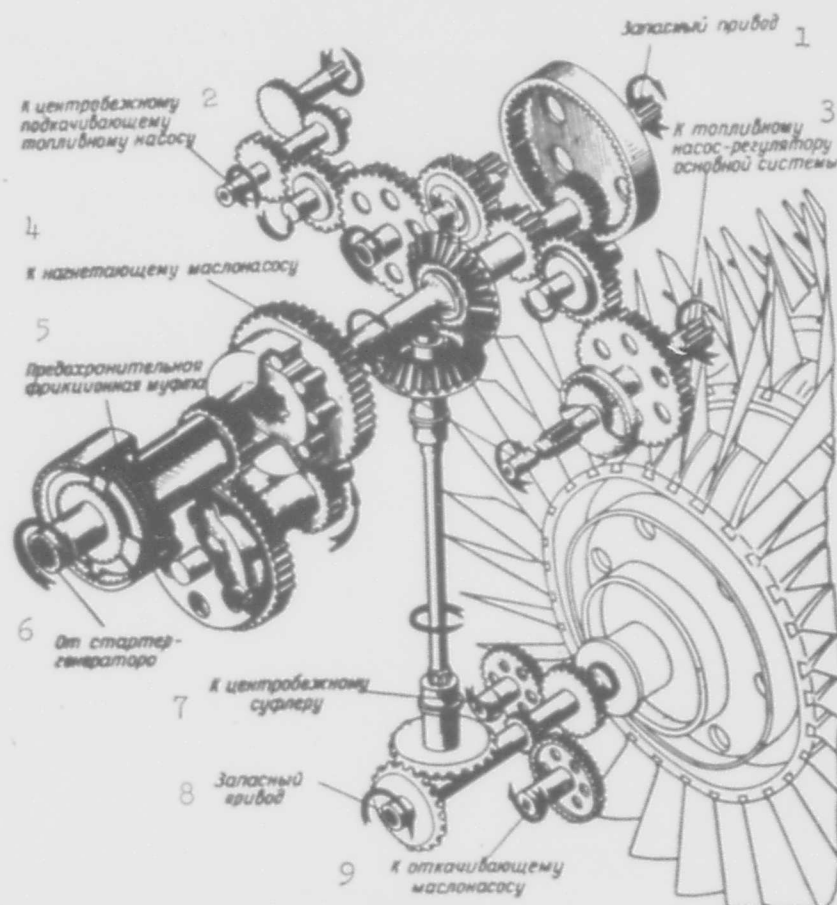
Fig. 157. Kinematic diagram of assembly drives in an engine with an axial compressor. 1) Spare drive; 2) to the centrifugal booster fuel pump; 3) to the fuel pump-regulator of the basic system; 4) to the pressure oil pump; 5) safety friction clutch; 6) from the starter generator; 7) to the centrifugal breather; 8) spare drive; 9) to the vacuum oil pump.
