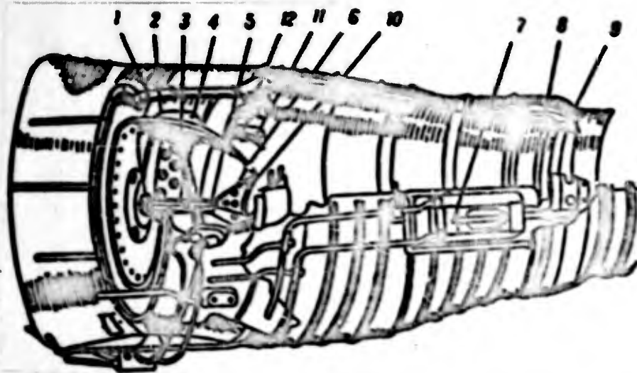
Fig. 127. Afterburner for TRD: 1) diffuser outside pipe; 2) inside cone; 3) stress-bearing rod; 4) streamlined strut; 5) starting (ignition) plug; 6) diaphragm; 7) hydraulic cylinder for flap control; 8) annular housing; 9) nozzle flap; 10) center flameholder; 11) annular flameholders; 12) nozzles.
