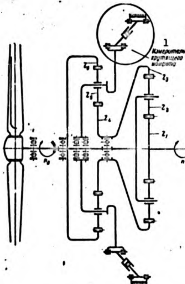
Fig. 184. Differential closed reduction gear for driving single propeller. 1) Torquemeter.
