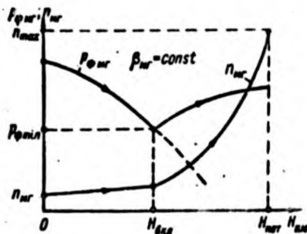
Fig. 288. Variation in minimum fuel pressure ahead of injectors and idle-running rotor speed with flight altitude in the presence of a direct-acting minimum-pressure valve.
