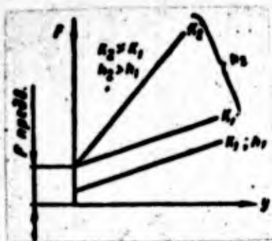
Fig. 236. Curves for sensing-element spring with various stiffnesses k and various positions of the adjusting mechanism (coordinate h ).
