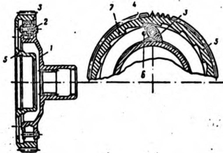
Fig. 317. Ratchet-type centrifugal clutch. 1) Driven portion of clutch; 2) dog axis; 3) dog; 4) spring; 5) driving portion of clutch; 6) stop; 7) angular tooth.
