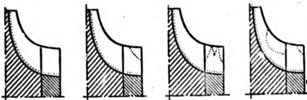
Fig. 58. Modes of coupled blade vibration of rotating guide-vane assembly and of the rotor of centrifugal compressor.
