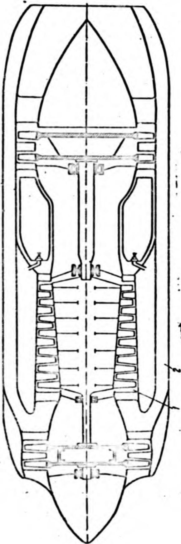
Fig. 3. Diagram of turbofan engine. 1) Inner (basic) duct; 2) outer duct.
