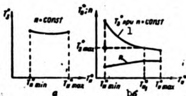
Fig. 218. Gas temperature T_3^* ahead of turbine nozzle-box assembly and rotor speed n as functions of stagnation temperature T_0^* at engine intake. T_{3\max}^* ) Maximum permissible gas temperature; T_{0\max}^* and T_{0\min}^* ) maximum and minimum possible air temperatures at engine intake, respectively; T_{01}^* ) value of T_0^* below which speed is restricted. 1) For.
