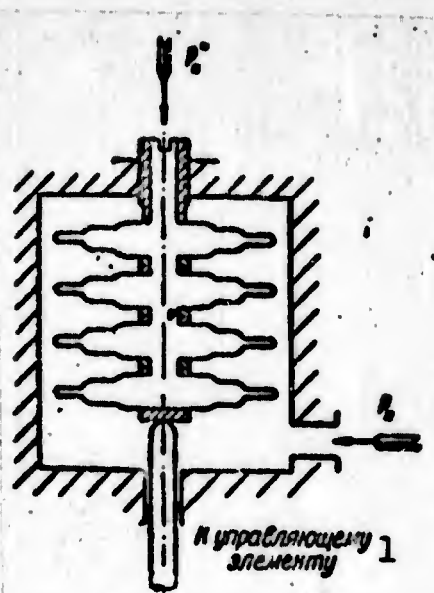
Fig. 248. Basic circuit of sensing element for air pressure drop. 1) To control element.
