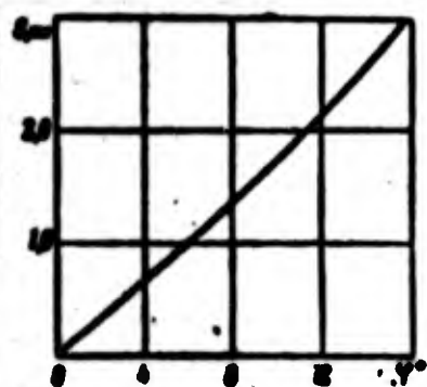
Fig. 202. Piston stroke S as a function of disk angle of inclination \phi .
