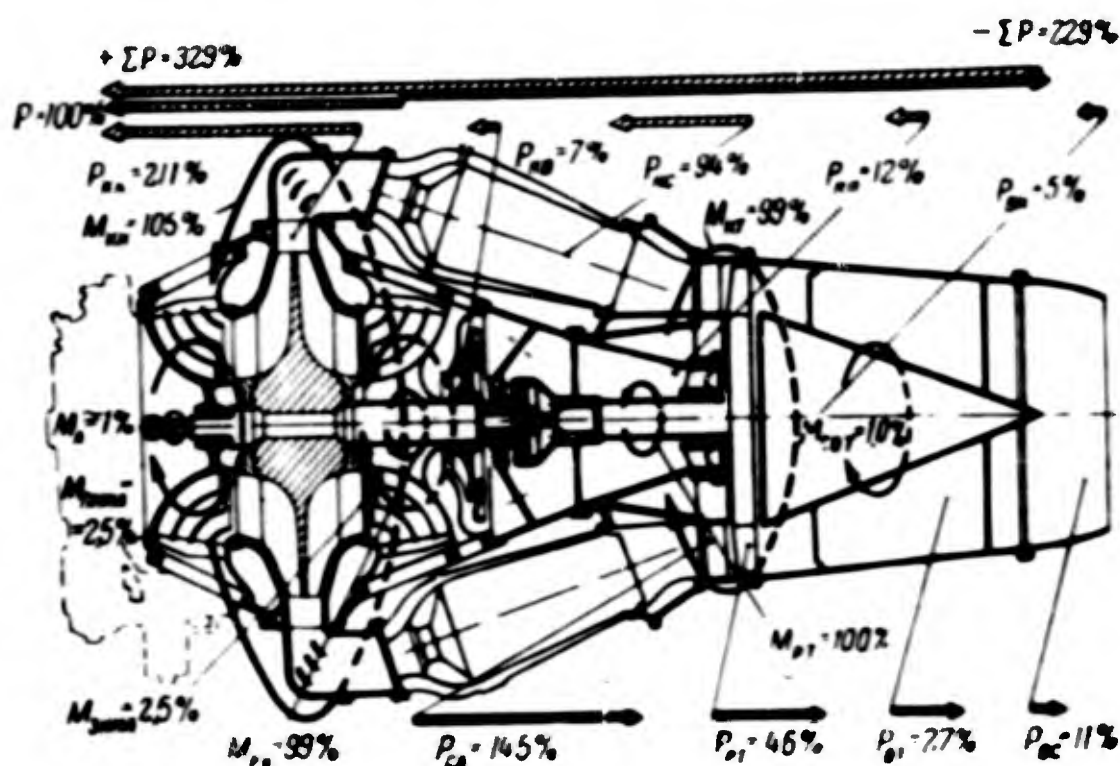
Fig. 134. The balance of axial forces and torques acting on the elements of the stress-bearing system of a turbojet [TRD] engine with a centrifugal compressor. (Based on percentage of the thrust force and torque on the turbine rotor for an engine with a centrifugal compressor, in the static operational regime with maximum rpm). P_{KK} ) axial force on compressor housing; P_{KV} ) axial force on fan housing; P_{KS} ) axial force on combustion chamber; P_{KP} ) axial force on bearing housing; P_{VK} ) axial force on inner cone; P_{SA} ) axial force on nozzle diaphragm; P_{RT} ) axial force on turbine rotor; P_{VT} ) axial force on outlet tube; P_{VS} ) axial force on outlet nozzle; M_A ) torque on assembly drive; M_K ) torque on compressor rotor; M_{RT} ) torque on turbine rotor; M_{PNNA} ) torque on forward fixed guide-vane assembly; M_{KK} ) torque on compressor housing; M_{ZNNA} ) torque on rear fixed guide-vane assembly; M_{KT} ) torque on turbine housing; M_{SVT} ) torque on the outlet tube struts.
