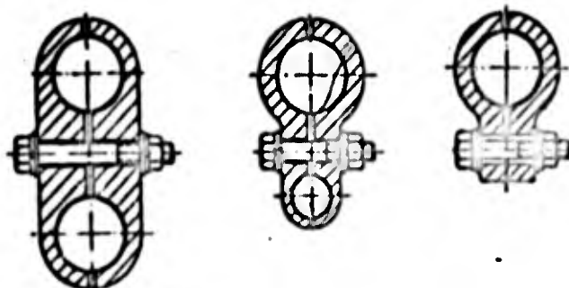
Fig. 176. Types of fasteners for attachment of oil ducts.
