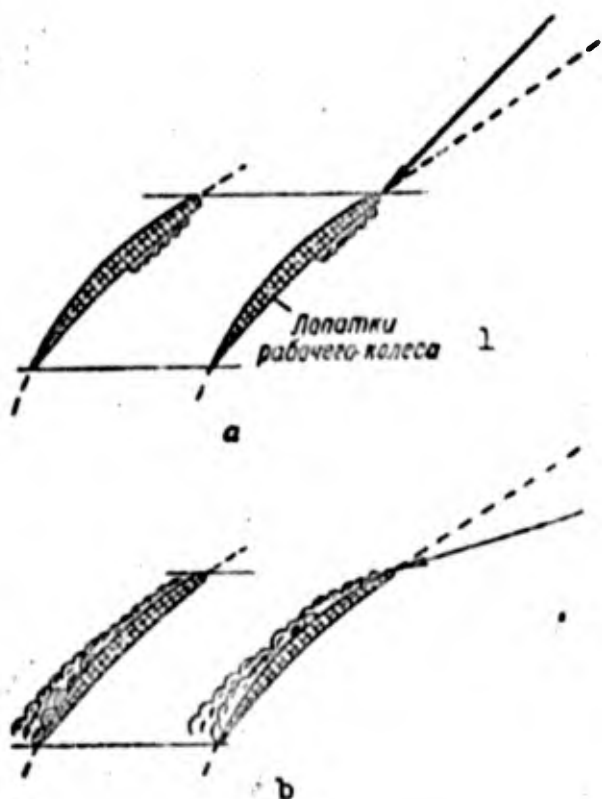
Fig. 48. Flow around the blades of compressor stages under unrated conditions. a) First stages; b) last stages (dashed line indicates the flow direction in the design [rated] regime). 1) Blade of rotor.
