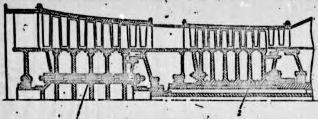
Fig. 12. Diagram of a two-spool axial compressor. 1) Low-pressure rotor; 2) high-pressure rotor.
