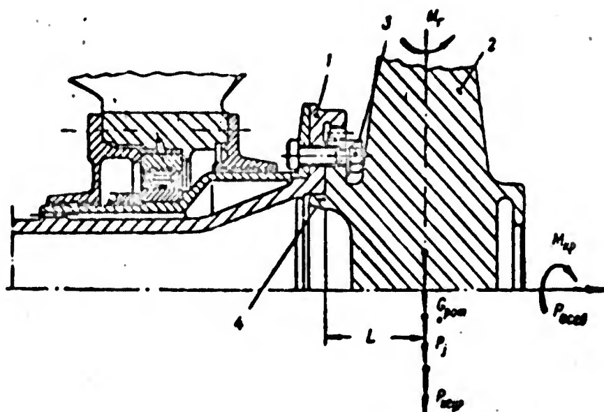
Fig. 75. Loads acting on the point of turbine disk coupling to the shaft. M_{kr} ) Turbine torque; G_{rot} ) rotor weight; P_j ) force of inertia; P_{neur} ) unbalanced centrifugal force; P_{osv} ) turbine axial force; M_g ) gyroscopic moment; 1) shaft flange; 2) turbine disk; 3) bolt; 4) collar.
