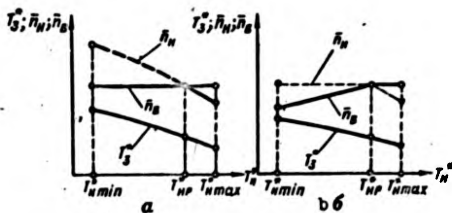
Fig. 222. Gas temperature T^*_3 and relative speeds of low-pressure rotor \bar{n}_L and high-pressure rotor \bar{n}_H as functions of temperature T^*_N . a) With \bar{n}_H constant; b) with restriction \bar{n}_L = 1 .
