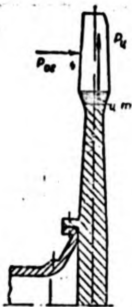
Fig. 71. Displacement of the center of disk rim gravity for purpose of countering the bending moment due to gas forces by a bending moment due to centrifugal forces. p_{ts} axial gas forces; p_{ts} centrifugal force;
