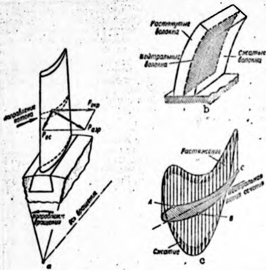
Fig. 18. Illustrations bearing on blade bending because of aerodynamic force. a) Diagram of action of aerodynamic force; b) diagram of bending of a flat plate; c) stresses acting on the blade cross section; P_{aer} aerodynamic force; P_{okr} and P_{os} circumferential and axial components of aerodynamic force, respectively; 1) Flow direction; 2) direction of rotation; 3) rotational axis; 4) fiber under tension; 5) neutral fiber; 6) fiber under compression; 7) tension; 8) neutral line of cross section; 9) compression.
