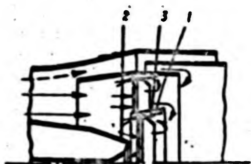
Fig. 128. Arrangement used to create flow-reversal zones by means of flameholders: 1) flameholder ring; 2) central flameholder; 3) nozzle.
