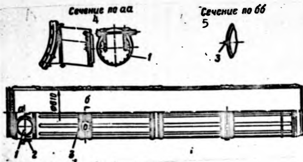
Fig. 122. Extension pipe: 1) gas-bypass gate valve; 2) drain; 3) pipe attachment fitting; 4) section through aa; 5) section through bb.
