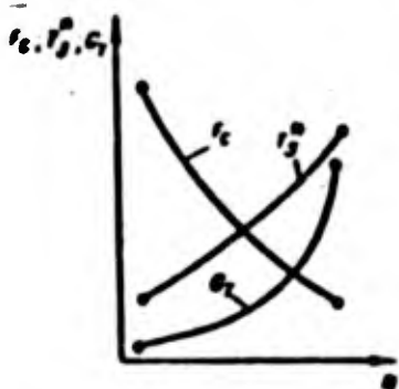
Fig. 219. Nozzle throat area F_5 , gas temperature T_3^* ahead of turbine nozzle-box assembly, and fuel flow rate G_t as functions of rotor speed n with optimum TRD control program.
