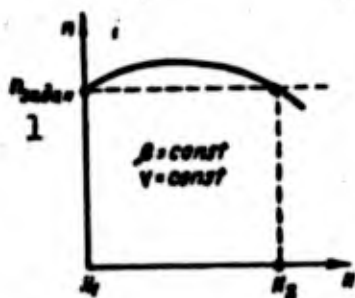
Fig. 276. Variation in speed with flight altitude for linear actual barostat characteristic. 1) n_{\text{zadan}}
