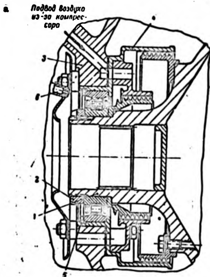
Fig. 161. Design of support with a single roller bearing. 1) Journal; 2) nut; 3) support housing; 4) cup; 5) spring ring; 6) oil injector; a) air feed from behind the compressor.
