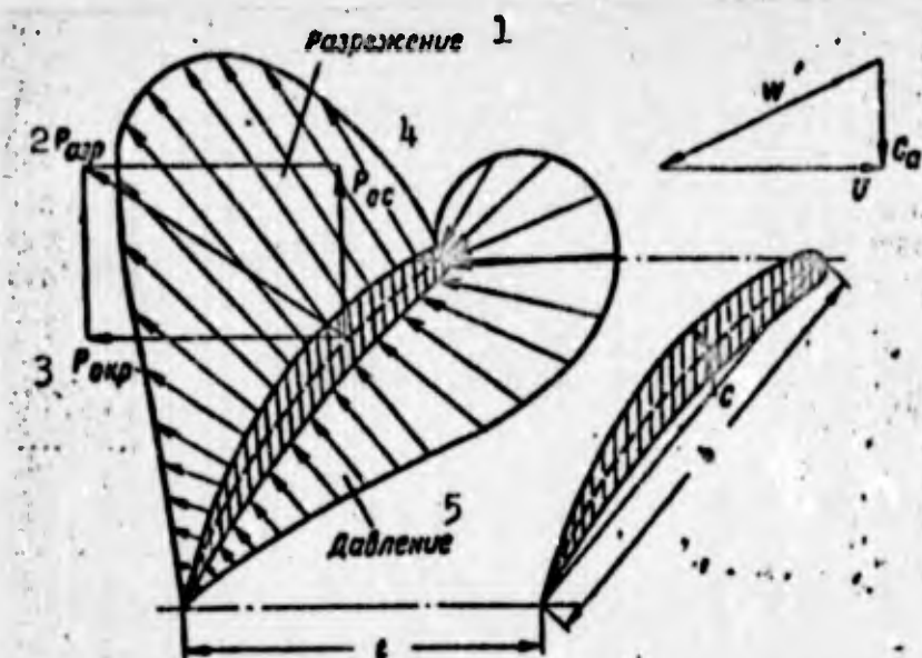
Fig. 10. Profile of the rotor blades of a subsonic stage. P_{aer} ) Aerodynamic force; P_{os} ) axial component; P_{okr} ) circumferential component; U ) circumferential speed; C_a ) axial speed; W ) relative speed; b ) chord; c ) thickness of profile; t ) pitch of blades; 1) Rarefaction; 2) P_{aer} ; 3) P_{okr} ; 4) P_{os} ; 5) pressure.
