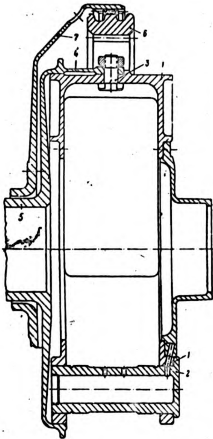
Fig. 194. Satellite carrier and large gear z_3 of reduction gear (a diagram of the reduction gear is shown in Fig. 185): 1) satellite carrier; 2) satellite shaft; 3) radial bulk; 4) flange of front propeller shaft; 5) shaft of front propeller; 6) gear z_3 ; 7) flange of rear propeller shaft.
