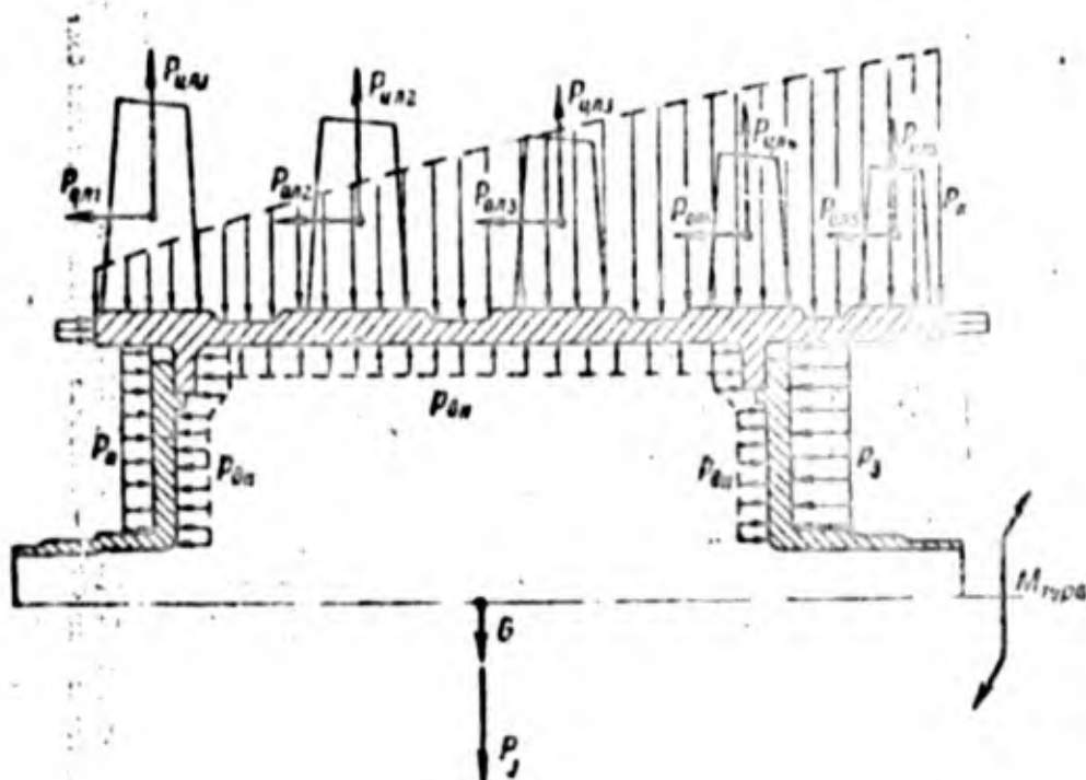
Fig. 31. Loading diagram of the compressor rotor. P_{tsl} ) Centrifugal blade forces; P_{ol} ) axial forces on the rotor blades; p_k ) air pressure in the flow passage; p_{vn} ) air pressure inside the rotor; p_p ) air pressure on the front end wall; p_z ) air pressure on the back end wall; G ) gravity force; P_j ) force of inertia; M_{turb} ) turbine moment.
