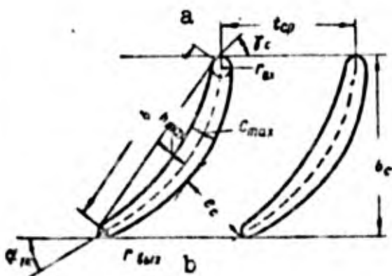
Fig. 81. Geometrical parameters of nozzle diaphragms. \alpha_{lk} ) Design angle of the gas flow outlet; e_c ) minimum channel width (see other designations in Fig. 66).
