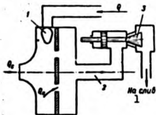
Fig. 216. Bypass injector: 1) tangential channel; 2) bypass channel; 3) distributor valve; Q_g ) flow through nozzle; Q_p ) bypassed fuel; Q ) total fuel flow. 1)
