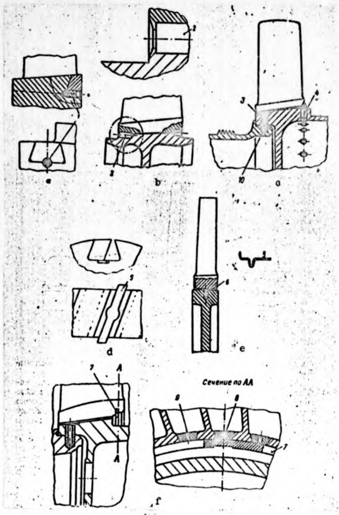
Fig. 17. Methods of attachment of blades to disks. a) Attachment by a screw; b) attachment by an axial : dowel; c) attachment by a radial dowel and plate lock; d) attachment by a plate lock with an enlargement; e) attachment by a wire lock; f) simultaneous attachment of all blades by a slotted spring ring; 1) screw; 2) axial dowel; 3) horn of plate lock; 4) radial dowel;
