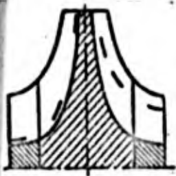
Fig. 56. Incidence of fatigue cracks in the vanes of a centrifugal compressor.
