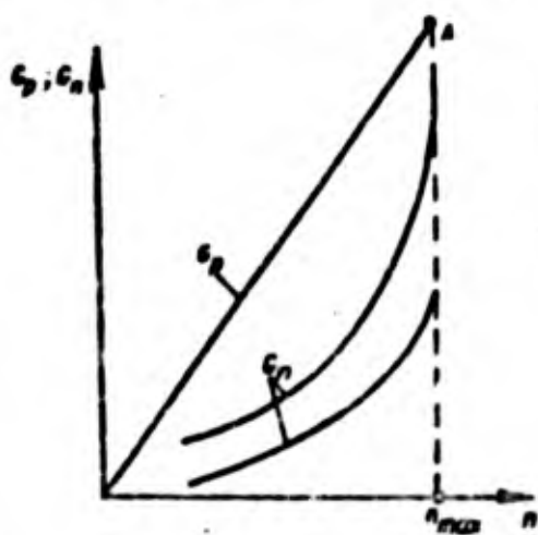
Fig. 227. Available fuel flow rate G_p from gear pump and required fuel flow rate G_r as functions of rotor speed n .
