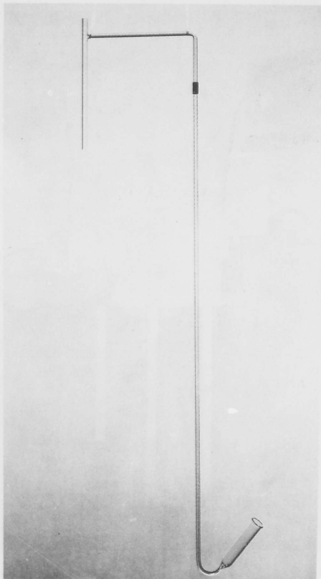
FIG. 1 VACUUM STABILITY TUBE AND MANOMETER
