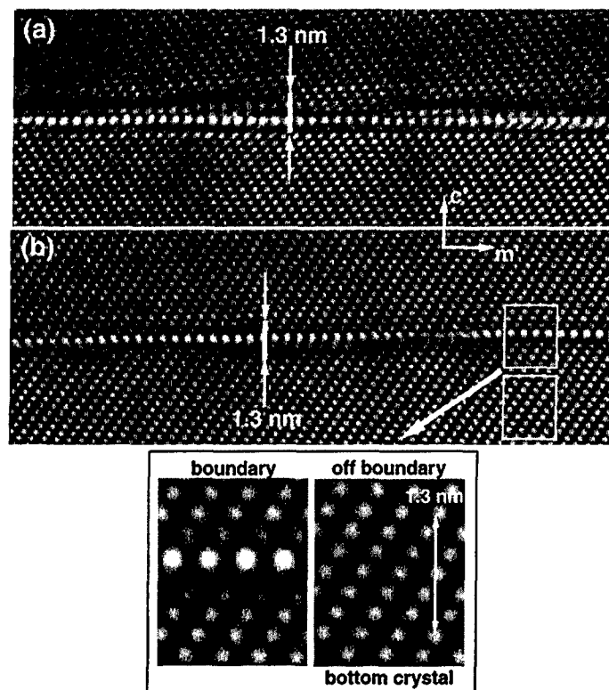
Fig. 10. HREM a -axis views of similar, narrow basal boundary sections designated as “dewetted” in Fig. 9. Although the boundaries are marked by distinct changes in contrast, both across and along the boundary (as discussed in the text), there is no resolvable evidence for a contiguous glassy film.
