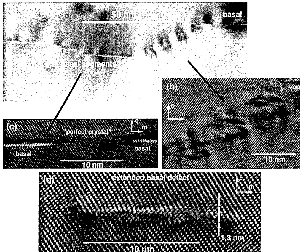
Fig. 11. TEM views of "steps" in the 3° basal tilt boundary also seen in Figs. 9 and 10. (a,b) For relatively large step heights, adjacent basal plane boundary sections are joined by a dislocation boundary segment, which is inclined by \sim 25^\circ to the median basal plane orientation. (c) For smaller ( \sim 1 to 2 nm) step heights, adjacent basal plane segments are separated by regions of "perfect" crystal. (d) a -axis HREM image of isolated basal plane boundary segment as seen in Figs. 10(a) and 10(b). Absence of interfacial glass film leads to conclusion that boundary contrast is due to dislocations and basal faults, which accommodate cation adsorbates from the glass phase.
