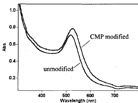
Figure 3. Comparative of UV-vis spectra of CMP modified gold nanoparticles and unmodified gold nanoparticles.
