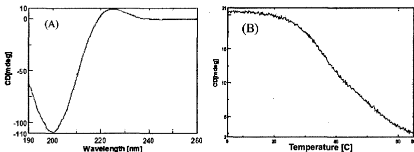
Figure 2. A: Circular dichroism spectrum of Cys-CMP; B: CD melting experiment of Cys-CMP.
