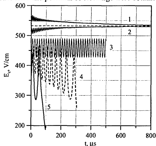
Fig.1. Relaxation (1-2) of electric field at the cathode ( R_c = 25 cm) for different \Delta U_{ps} = U_{ps}^*(p) - U_{ps} and auto-oscillation (3) Decaying regimes (curves 4-5) p = 3.5 Torr, and different power supply voltages U_{ps} .
