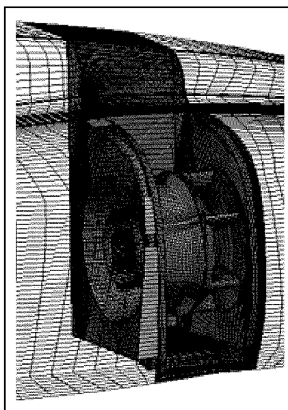
Figure 26: Hexahedral mesh on side-facing helicopter inlet
