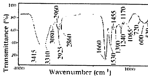
Fig. 8. Characteristic IR bands of artificial cobweb
