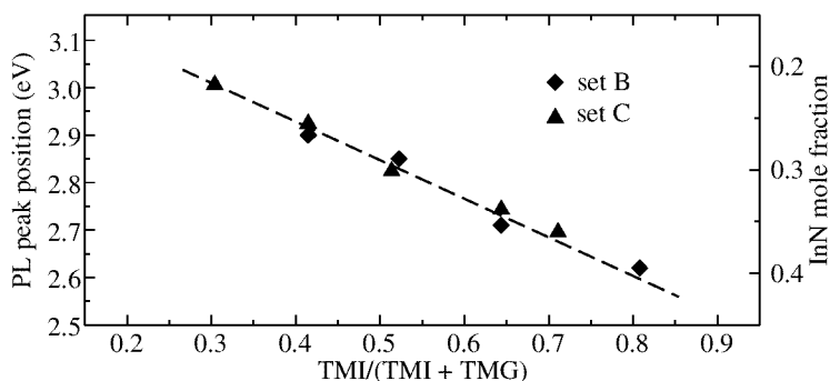
Fig. 1. 77 K PL peak position versus TMI/(TMI+TMG) mole flow ratio for samples from sets B and C.
