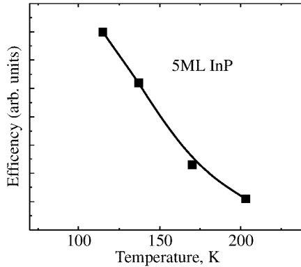
Fig. 2. Temperature dependence of quantum efficiency of 5 ML InP NSI, P = 50 \text{ W/cm}^2 .
