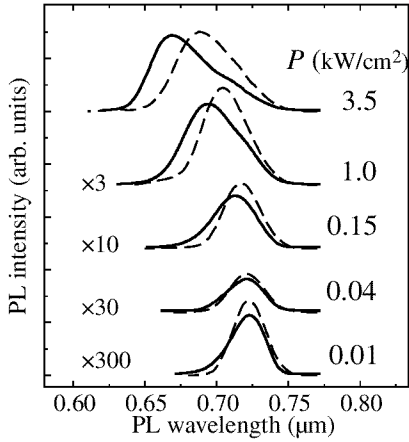
Fig. 3. 77 K PL spectra of 3 ML (solid line) and 5 ML (dashed line) InP NSIs at different excitation level.
