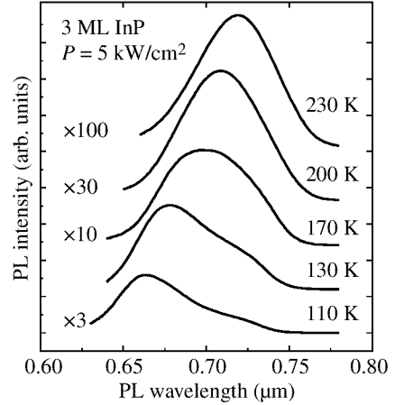
Fig. 4. PL spectra of 3 ML InP NSIs at high excitation level ( 5 \text{ kW/cm}^2 ) for different measuring temperatures.
