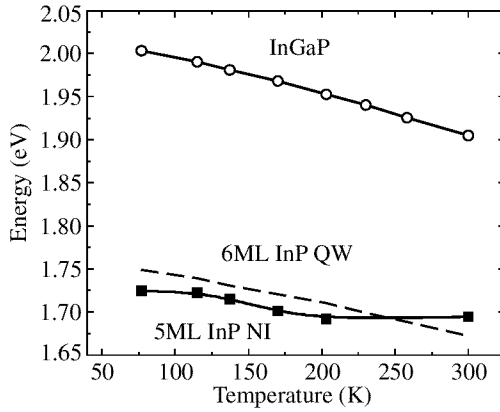
Fig. 1. PL temperature dependence for 5 ML InP NSI (solid square), InGaP matrix (open circle) and 6 ML Quantum Well (dash line), P = 50 \text{ W/cm}^2 .
